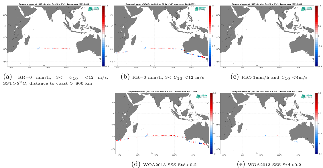
Figure 14: Temporal mean gridded over spatial boxes of size 1^\circ \times 1^\circ of \Delta SSS (SMOS SSS L2 v700 (ESA) - TSG (CSIC-UTM)) for 5 different subdatasets corresponding to:RR=0 mm/h, 3 < U_{10} < 12 m/s, SST>5°C, distance to coast > 800 km (a), RR=0 mm/h, 3 < U_{10} < 12 m/s (b), RR>1mm/h and U_{10} < 4 m/s (c), WOA2013 SSS Std<0.2 (d), WOA2013 SSS Std>0.2 (e).
