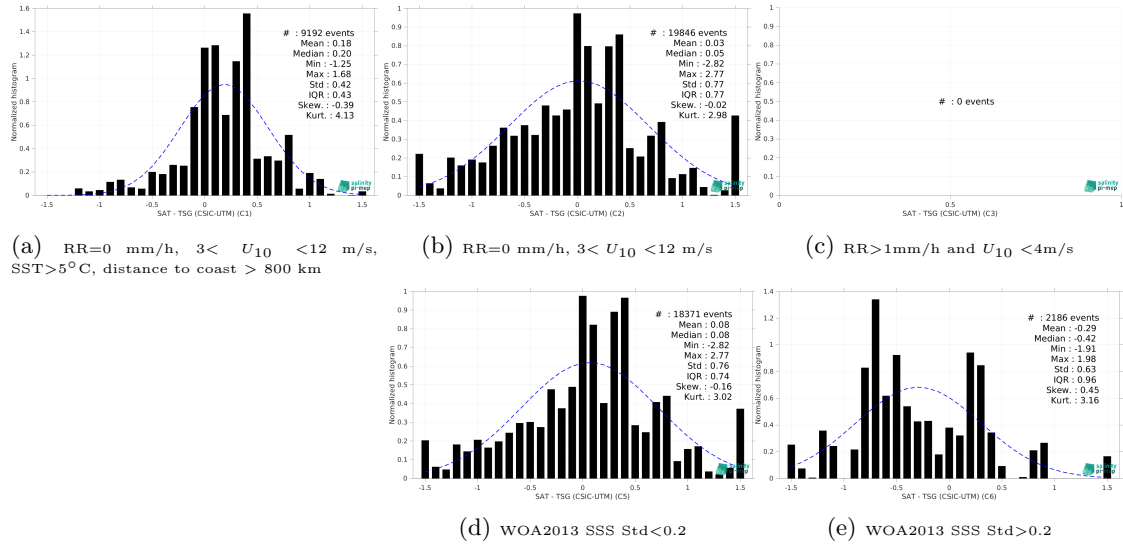
Figure 15: Normalized histogram of \Delta\text{SSS} (SMOS SSS L2 v700 (ESA) - TSG (CSIC-UTM)) for 5 different subdatasets corresponding to: RR=0 mm/h, 3 < U_{10} < 12 m/s, SST>5°C, distance to coast > 800 km (a), RR=0 mm/h, 3 < U_{10} < 12 m/s (b), RR>1mm/h and U_{10} < 4 m/s (c), WOA2013 SSS Std<0.2 (d), WOA2013 SSS Std>0.2 (e).
