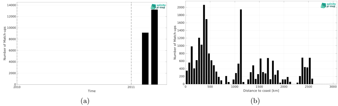
Figure 2: Number of match-ups between TSG (CSIC-UTM) and SMOS SSS L2 v700 (ESA) SSS as a function of time (a) and as function of the distance to coast (b) over the Indian Ocean Pi-MEP region and for the full satellite product period.
