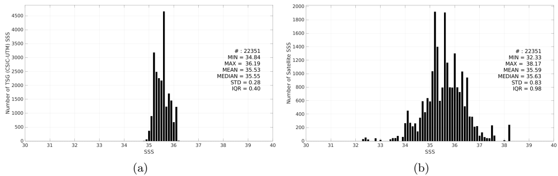
Figure 3: Histograms of SSS from TSG (CSIC-UTM) (a) and SMOS SSS L2 v700 (ESA) (b) considering all match-up pairs per bins of 0.1 over the Indian Ocean Pi-MEP region and for the full satellite product period.
