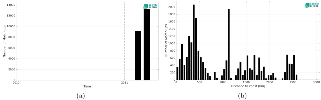
Figure 1: Number of match-ups between TSG (CSIC-UTM) and SMOS SSS L2 v700 (ESA) SSS as a function of time (a) and as function of the distance to coast (b) over the Indian Ocean Pi-MEP region and for the full satellite product period.
