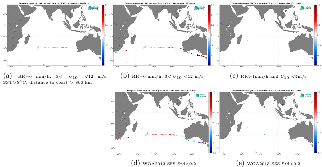
Figure 12: Temporal mean gridded over spatial boxes of size 1^\circ \times 1^\circ of \Delta SSS (SMOS SSS L2 v700 (ESA) - TSG (CSIC-UTM)) for 5 different subdatasets corresponding to:RR=0 mm/h, 3 < U_{10} < 12 m/s, SST >5^\circ\text{C} , distance to coast > 800 km (a), RR=0 mm/h, 3 < U_{10} < 12 m/s (b), RR >1 mm/h and U_{10} < 4 m/s (c), WOA2013 SSS Std <0.2 (d), WOA2013 SSS Std >0.2 (e).
