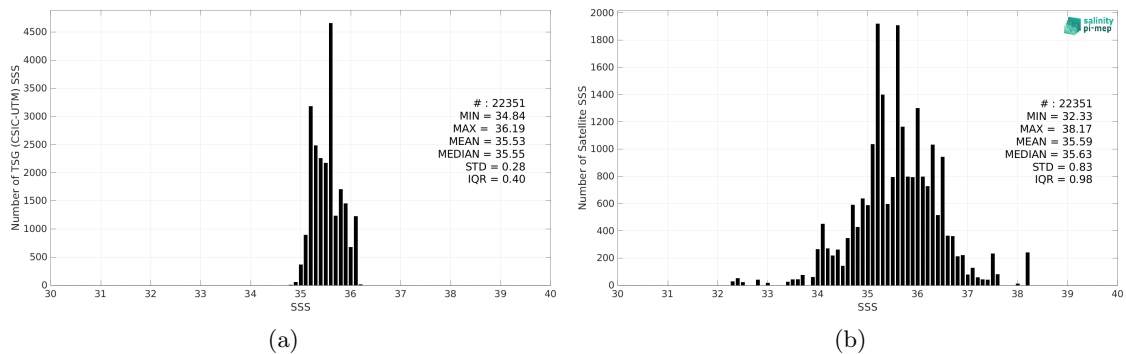
Figure 2: Histograms of SSS from TSG (CSIC-UTM) (a) and SMOS SSS L2 v700 (ESA) (b) considering all match-up pairs per bins of 0.1 over the Indian Ocean Pi-MEP region and for the full satellite product period.
