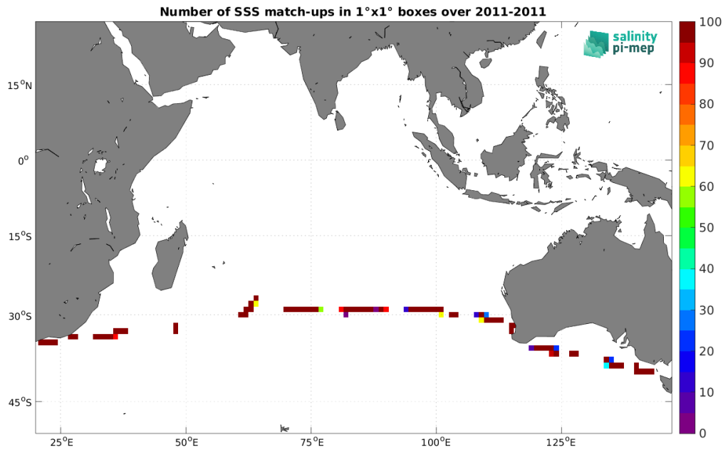
Figure 4: Number of SSS match-ups between TSG (CSIC-UTM) SSS and the SMOS SSS L2 v700 (ESA) SSS product for the Indian Ocean Pi-MEP region over 1^\circ \times 1^\circ boxes and for the full satellite product period.
