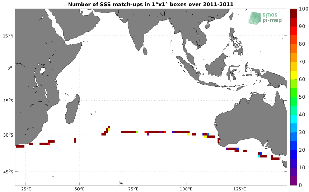
Figure 4: Number of SSS match-ups between TSG (CSIC-UTM) SSS and the SMOS SSS L2 v700 (ESA) SSS product for the Indian Ocean Pi-MEP region over 1^\circ \times 1^\circ boxes and for the full satellite product period.
