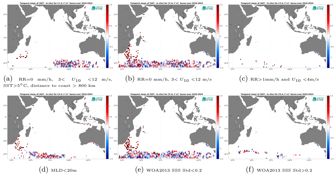
Figure 14: Temporal mean gridded over spatial boxes of size 1^\circ \times 1^\circ of \Delta\text{SSS} (SMOS SSS L2 v700 (ESA) - Marine mammals) for 6 different subdatasets corresponding to:RR=0 mm/h, 3 < U_{10} < 12 m/s, SST>5°C, distance to coast > 800 km (a), RR=0 mm/h, 3 < U_{10} < 12 m/s (b), RR>1mm/h and U_{10} < 4 m/s (c),MLD<20m (d),WOA2013 SSS Std<0.2 (e),WOA2013 SSS Std>0.2 (f).
