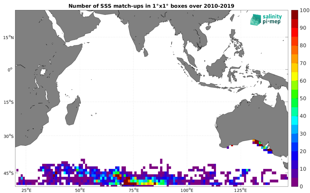
Figure 4: Number of SSS match-ups between Marine mammals SSS and the SMOS SSS L2 v700 (ESA) SSS product for the Indian Ocean Pi-MEP region over 1^\circ \times 1^\circ boxes and for the full satellite product period.
