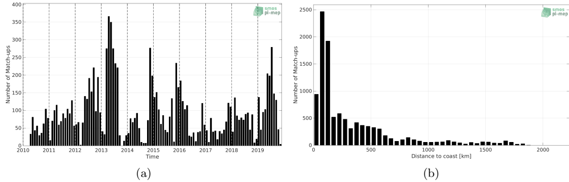
Figure 1: Number of match-ups between Marine mammals and SMOS SSS L2 v700 (ESA) SSS as a function of time (a) and as function of the distance to coast (b) over the Indian Ocean Pi-MEP region and for the full satellite product period.
