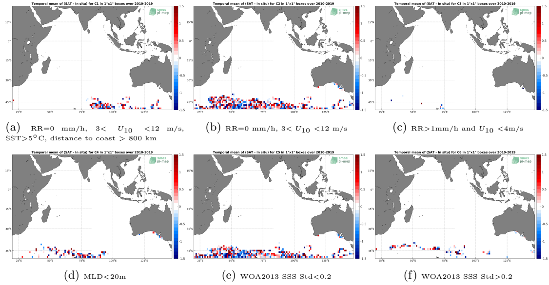
Figure 12: Temporal mean gridded over spatial boxes of size 1^\circ \times 1^\circ of \Delta SSS (SMOS SSS L2 v700 (ESA) - Marine mammals) for 6 different subdatasets corresponding to: RR=0 mm/h, 3 < U_{10} < 12 m/s, SST > 5^\circ C , distance to coast > 800 km (a), RR=0 mm/h, 3 < U_{10} < 12 m/s (b), RR > 1 mm/h and U_{10} < 4 m/s (c), MLD < 20 m (d), WOA2013 SSS Std < 0.2 (e), WOA2013 SSS Std > 0.2 (f).
