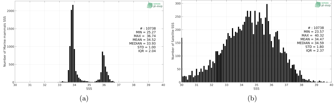
Figure 2: Histograms of SSS from Marine mammals (a) and SMOS SSS L2 v700 (ESA) (b) considering all match-up pairs per bins of 0.1 over the Indian Ocean Pi-MEP region and for the full satellite product period.
