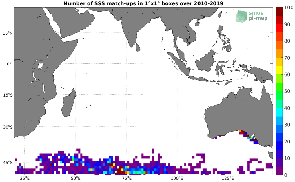
Figure 4: Number of SSS match-ups between Marine mammals SSS and the SMOS SSS L2 v700 (ESA) SSS product for the Indian Ocean Pi-MEP region over 1^\circ \times 1^\circ boxes and for the full satellite product period.
