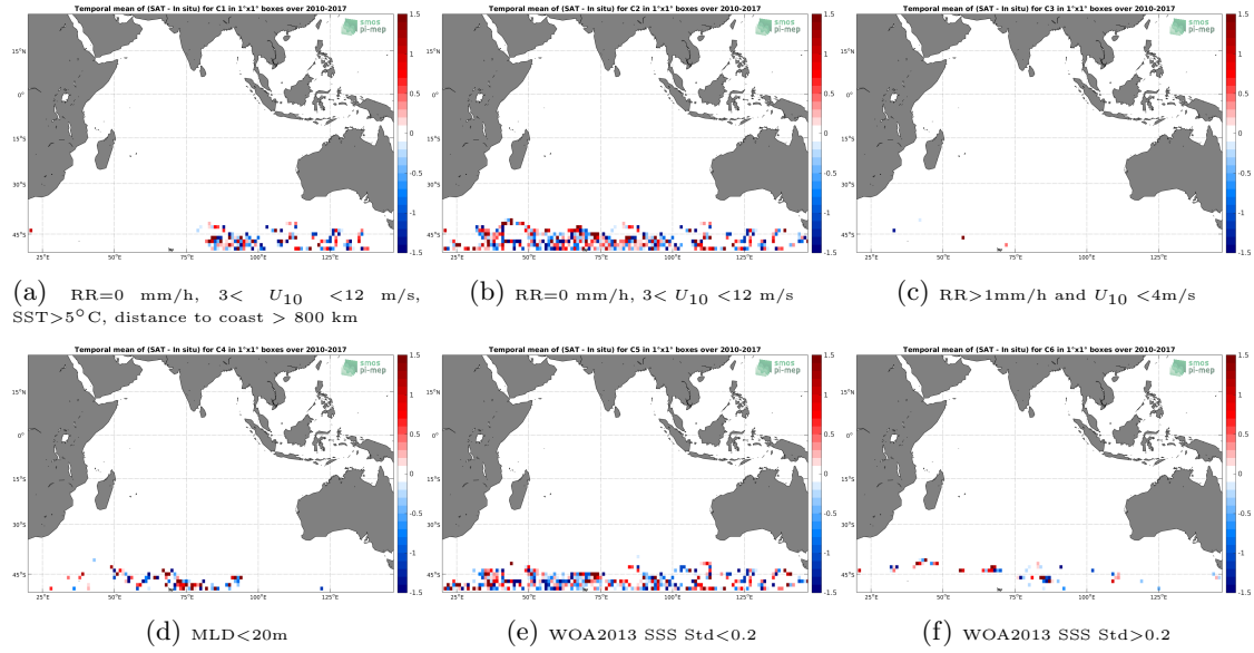
Figure 12: Temporal mean gridded over spatial boxes of size 1^{\circ}\times 1^{\circ} of \Delta\text{SSS} (SMOS SSS L2 v700 (ESA) - Sea mammals) for 6 different subdatasets corresponding to: \text{RR}=0 mm/h, 3 < U_{10} < 12 m/s, \text{SST} > 5^{\circ}\text{C} , distance to coast > 800 km (a), \text{RR}=0 mm/h, 3 < U_{10} < 12 m/s (b), \text{RR} > 1\text{mm/h} and U_{10} < 4\text{m/s} (c), \text{MLD} < 20\text{m} (d), \text{WOA2013 SSS Std} < 0.2 (e), \text{WOA2013 SSS Std} > 0.2 (f).
