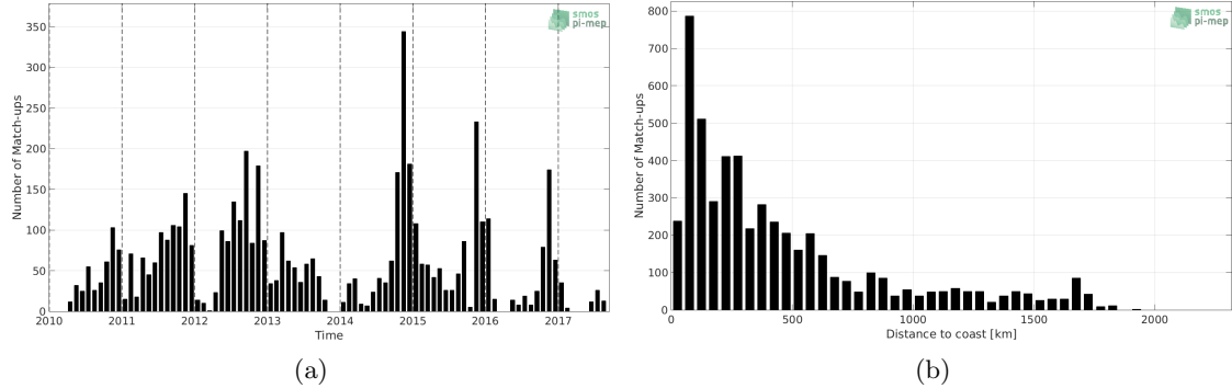
Figure 1: Number of match-ups between Sea mammals and SMOS SSS L2 v700 (ESA) SSS as a function of time (a) and as function of the distance to coast (b) over the Indian Ocean Pi-MEP region and for the full satellite product period.
