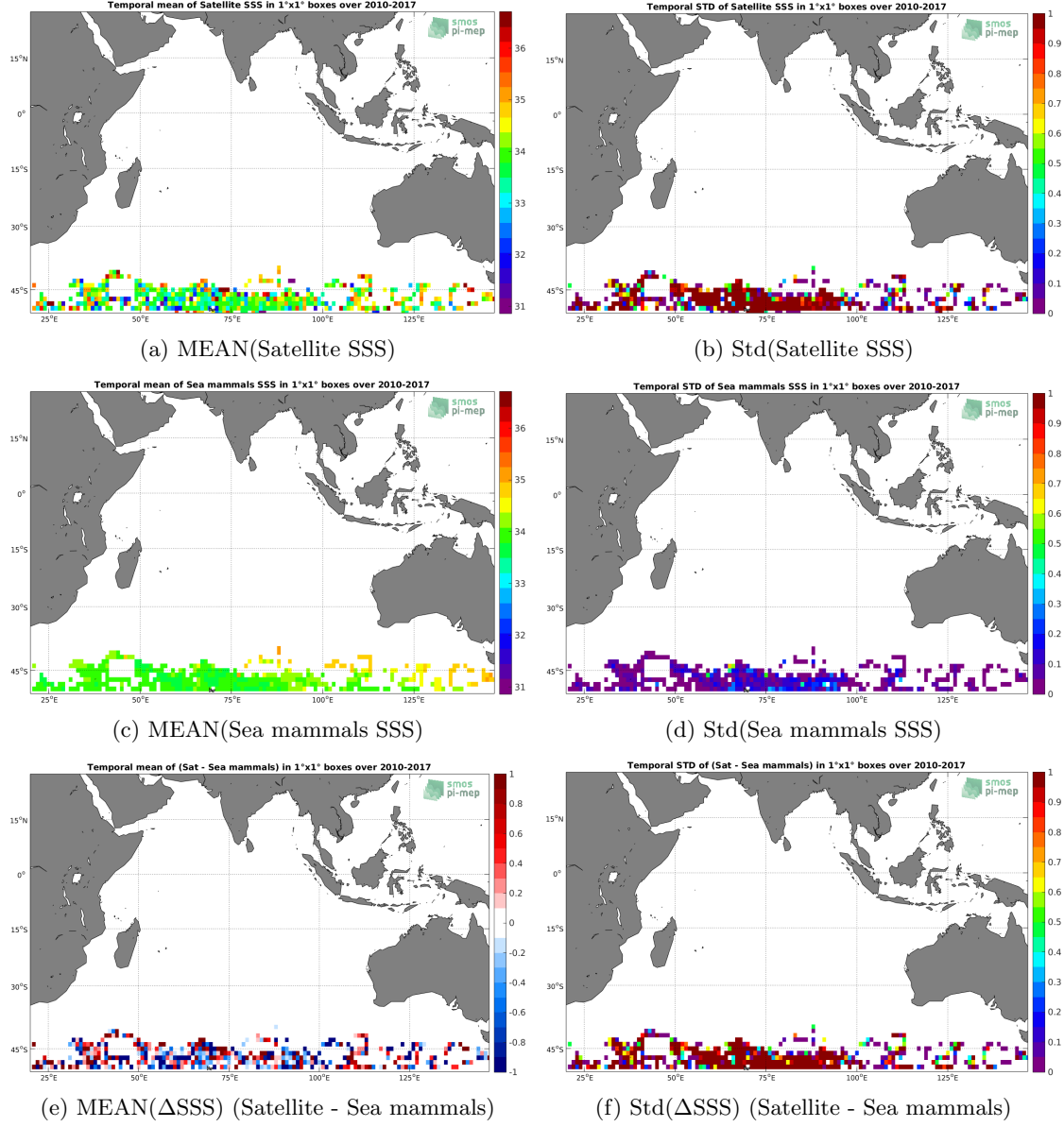
Figure 6: Temporal mean (left) and Std (right) of SSS from SMOS SSS L2 v700 (ESA) (top), Sea mammals (middle), and of \Delta SSS (Satellite - Sea mammals). Only match-up pairs are used to generate these maps.
