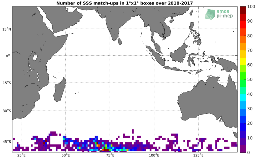
Figure 4: Number of SSS match-ups between Sea mammals SSS and the SMOS SSS L2 v700 (ESA) SSS product for the Indian Ocean Pi-MEP region over 1^\circ \times 1^\circ boxes and for the full satellite product period.
