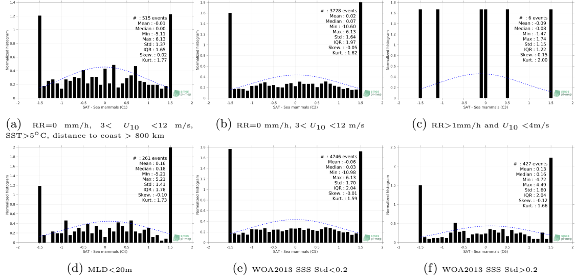
Figure 13: Normalized histogram of \Delta SSS (SMOS SSS L2 v700 (ESA) - Sea mammals) for 6 different subdatasets corresponding to: RR=0 mm/h, 3 < U_{10} < 12 m/s, SST>5°C, distance to coast > 800 km (a), RR=0 mm/h, 3 < U_{10} < 12 m/s (b), RR>1mm/h and U_{10} < 4 m/s (c), MLD<20m (d), WOA2013 SSS Std<0.2 (e), WOA2013 SSS Std>0.2 (f).
