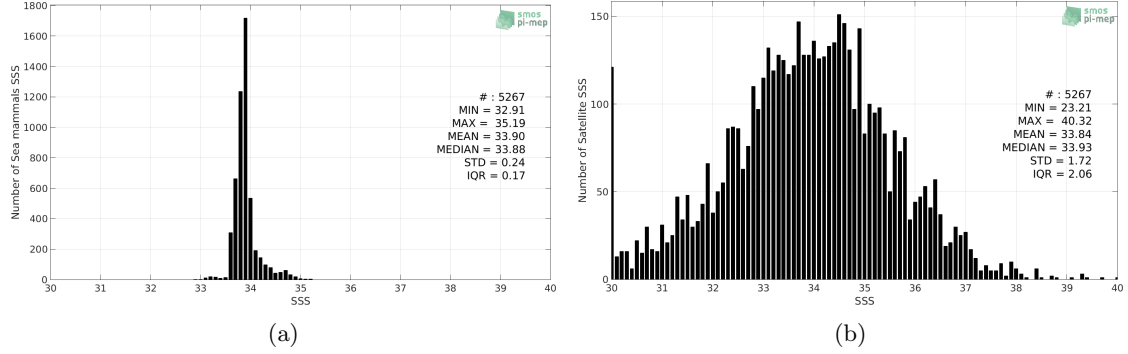
Figure 2: Histograms of SSS from Sea mammals (a) and SMOS SSS L2 v700 (ESA) (b) considering all match-up pairs per bins of 0.1 over the Indian Ocean Pi-MEP region and for the full satellite product period.
