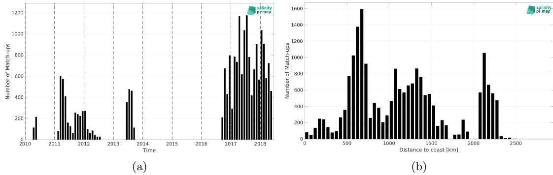
Figure 1: Number of match-ups between Surface drifters and SMOS SSS L2 v700 (ESA) SSS as a function of time (a) and as function of the distance to coast (b) over the Indian Ocean Pi-MEP region and for the full satellite product period.
