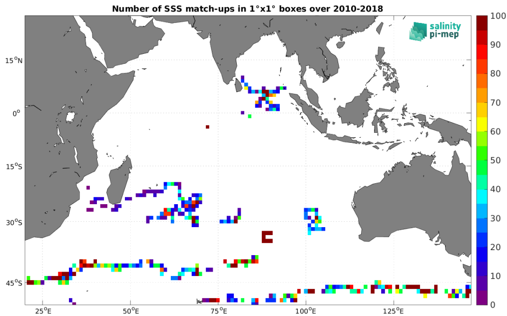
Figure 3: Number of SSS match-ups between Surface drifters SSS and the SMOS SSS L2 v700 (ESA) SSS product for the Indian Ocean Pi-MEP region over 1^\circ \times 1^\circ boxes and for the full satellite product period.
