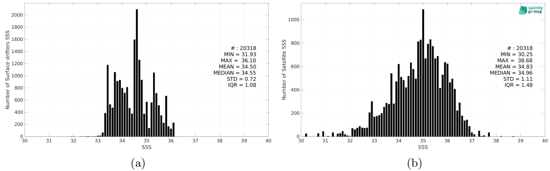
Figure 2: Histograms of SSS from Surface drifters (a) and SMOS SSS L2 v700 (ESA) (b) considering all match-up pairs per bins of 0.1 over the Indian Ocean Pi-MEP region and for the full satellite product period.
