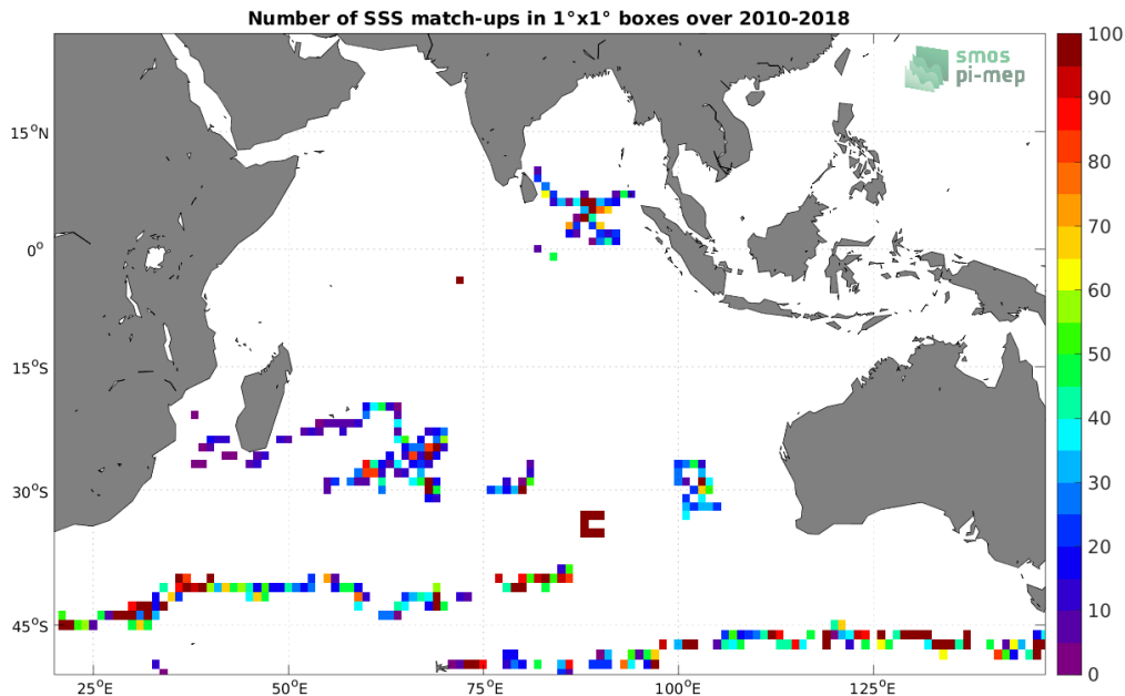
Figure 3: Number of SSS match-ups between Surface drifters SSS and the SMOS SSS L2 v700 (ESA) SSS product for the Indian Ocean Pi-MEP region over 1^\circ \times 1^\circ boxes and for the full satellite product period.
