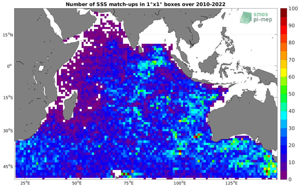
Figure 4: Number of SSS match-ups between Argo SSS and the SMOS SSS L2 v700 (ESA) SSS product for the Indian Ocean Pi-MEP region over 1^{\circ} \times 1^{\circ} boxes and for the full satellite product period.
