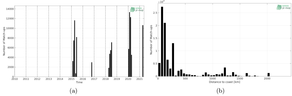
Figure 1: Number of match-ups between TSG (SAMOS) and SMOS SSS L2 v662 (ESA) SSS as a function of time (a) and as function of the distance to coast (b) over the Indian Ocean Pi-MEP region and for the full satellite product period.
