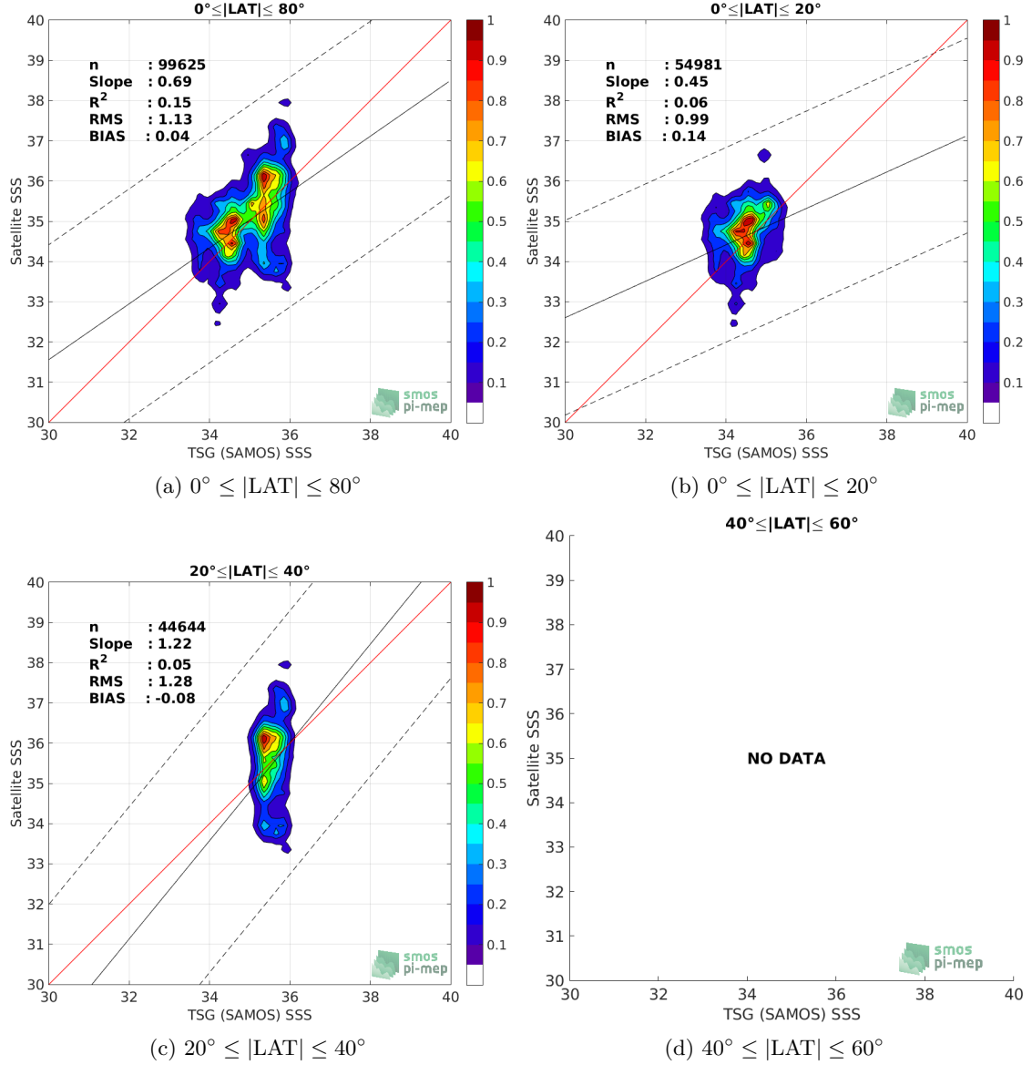
Figure 9: Contour maps of the concentration of SMOS SSS L2 v662 (ESA) SSS (y-axis) versus TSG (SAMOS) SSS (x-axis) at match-up pairs for different latitude bands. For each plot, the red line shows x=y . The black thin and dashed lines indicate a linear fit through the data cloud and the \pm 95\% confidence levels, respectively. The number match-up pairs n , the slope and R^2 coefficient of the linear fit, the root mean square (RMS) and the mean bias between satellite and in situ data are indicated for each latitude band in each plots.
