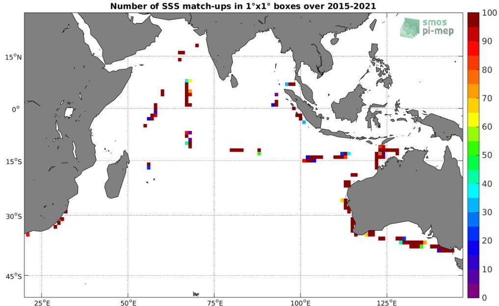
Figure 4: Number of SSS match-ups between TSG (SAMOS) SSS and the SMOS SSS L2 v662 (ESA) SSS product for the Indian Ocean Pi-MEP region over 1^\circ \times 1^\circ boxes and for the full satellite product period.
