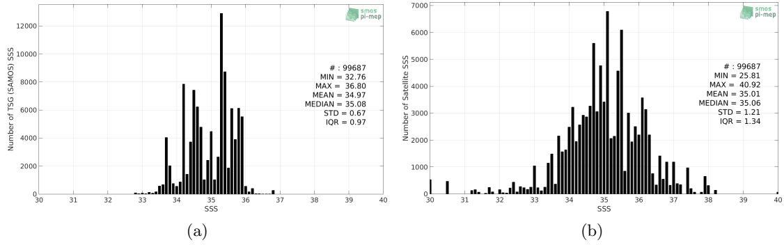
Figure 2: Histograms of SSS from TSG (SAMOS) (a) and SMOS SSS L2 v662 (ESA) (b) considering all match-up pairs per bins of 0.1 over the Indian Ocean Pi-MEP region and for the full satellite product period.
