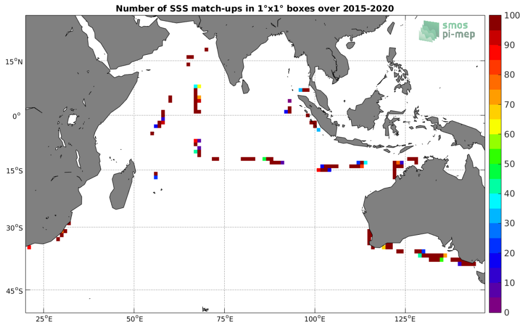
Figure 4: Number of SSS match-ups between TSG-SAMOS SSS and the SMOS L2 v662 (ESA) SSS product for the Indian Ocean Pi-MEP region over 1°x1° boxes and for the full satellite product period.
