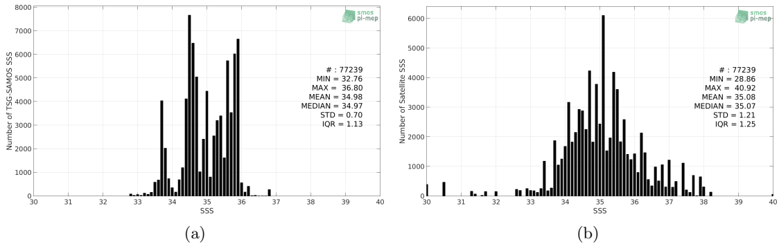
Figure 2: Histograms of SSS from TSG-SAMOS (a) and SMOS L2 v662 (ESA) (b) considering all match-up pairs per bins of 0.1 over the Indian Ocean Pi-MEP region and for the full satellite product period.
