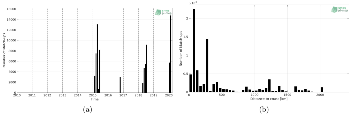
Figure 1: Number of match-ups between TSG-SAMOS and SMOS L2 v662 (ESA) SSS as a function of time (a) and as function of the distance to coast (b) over the Indian Ocean Pi-MEP region and for the full satellite product period.
