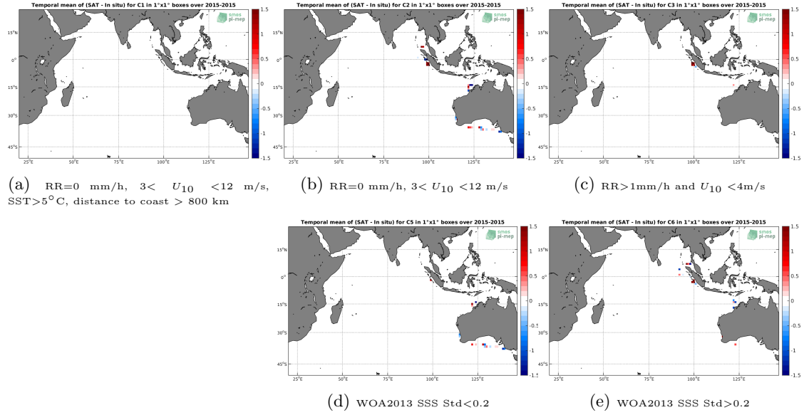
Figure 12: Temporal mean gridded over spatial boxes of size 1^\circ \times 1^\circ of \Delta SSS (SMOS-L2-DPGS-v662 - TSG-SAMOS) for 5 different subdatasets corresponding to: RR=0 mm/h, 3 < U_{10} < 12 m/s, SST >5^\circ C, distance to coast > 800 km (a), RR=0 mm/h, 3 < U_{10} < 12 m/s (b), RR >1 mm/h and U_{10} < 4 m/s (c), WOA2013 SSS Std <0.2 (d), WOA2013 SSS Std >0.2 (e).
