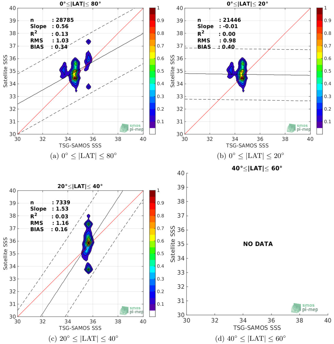
Figure 9: Contour maps of the concentration of SMOS-L2-DPGS-v662 SSS (y-axis) versus TSG-SAMOS SSS (x-axis) at match-up pairs for different latitude bands. For each plot, the red line shows x=y . The black thin and dashed lines indicate a linear fit through the data cloud and the \pm 95\% confidence levels, respectively. The number match-up pairs n , the slope and R^2 coefficient of the linear fit, the root mean square (RMS) and the mean bias between satellite and in situ data are indicated for each latitude band in each plots.
