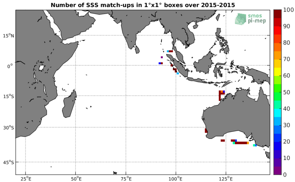
Figure 4: Number of SSS match-ups between TSG-SAMOS SSS and the SMOS-L2-DPGS-v662 SSS product for the Indian Ocean Pi-MEP region over 1°x1° boxes and for the full satellite product period.
