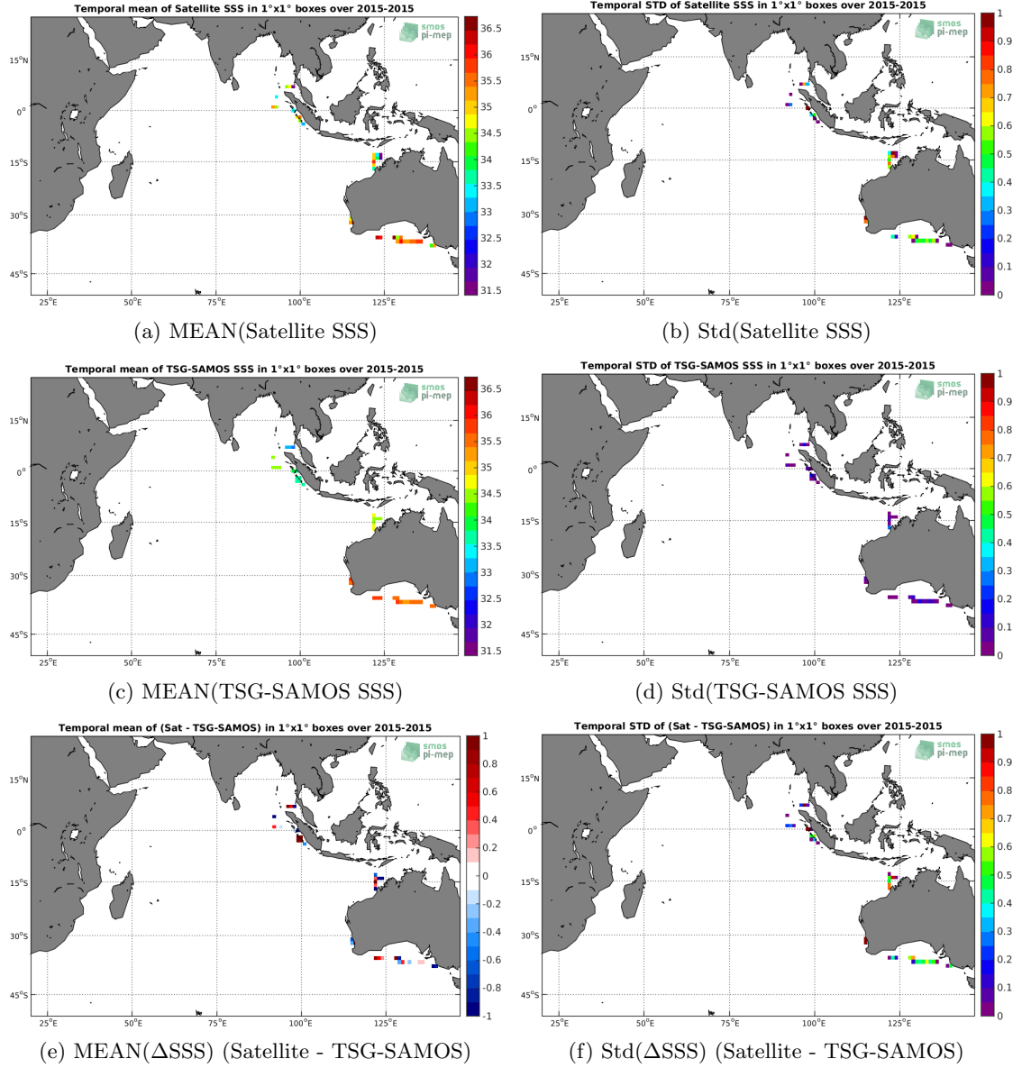
Figure 6: Temporal mean (left) and Std (right) of SSS from SMOS-L2-DPGS-v662 (top), TSG-SAMOS (middle), and of \Delta SSS (Satellite - TSG-SAMOS). Only match-up pairs are used to generate these maps.
