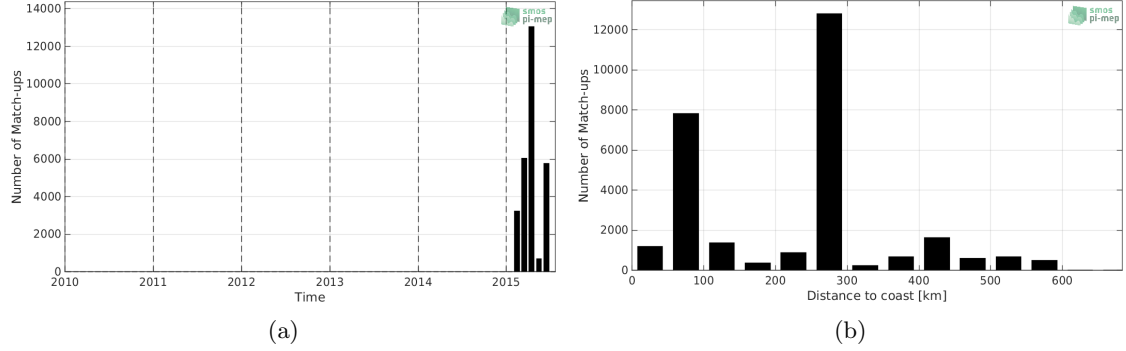
Figure 1: Number of match-ups between TSG-SAMOS and SMOS-L2-DPGS-v662 SSS as a function of time (a) and as function of the distance to coast (b) over the Indian Ocean Pi-MEP region and for the full satellite product period.
