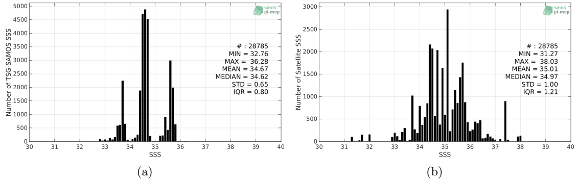
Figure 2: Histograms of SSS from TSG-SAMOS (a) and SMOS-L2-DPGS-v662 (b) considering all match-up pairs per bins of 0.1 over the Indian Ocean Pi-MEP region and for the full satellite product period.
