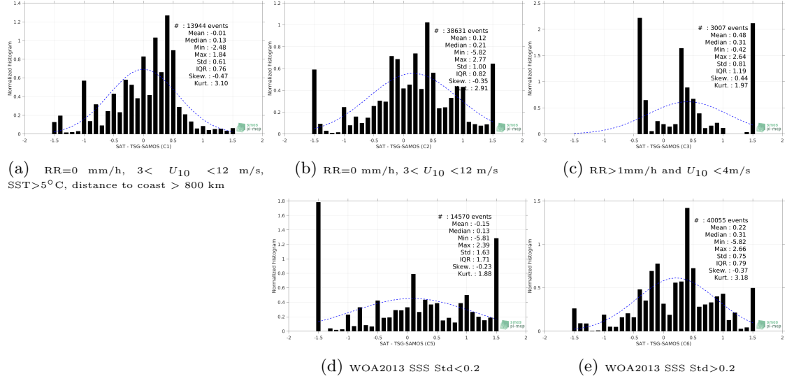
Figure 13: Normalized histogram of \Delta\text{SSS} (SMOS-L2-DPGS-v662 - TSG-SAMOS) for 5 different subdatasets corresponding to: RR=0 mm/h, 3 < U_{10} < 12 m/s, SST > 5^{\circ}\text{C} , distance to coast > 800 km (a), RR=0 mm/h, 3 < U_{10} < 12 m/s (b), RR > 1\text{mm/h} and U_{10} < 4\text{m/s} (c), WOA2013 SSS Std < 0.2 (d), WOA2013 SSS Std > 0.2 (e).
