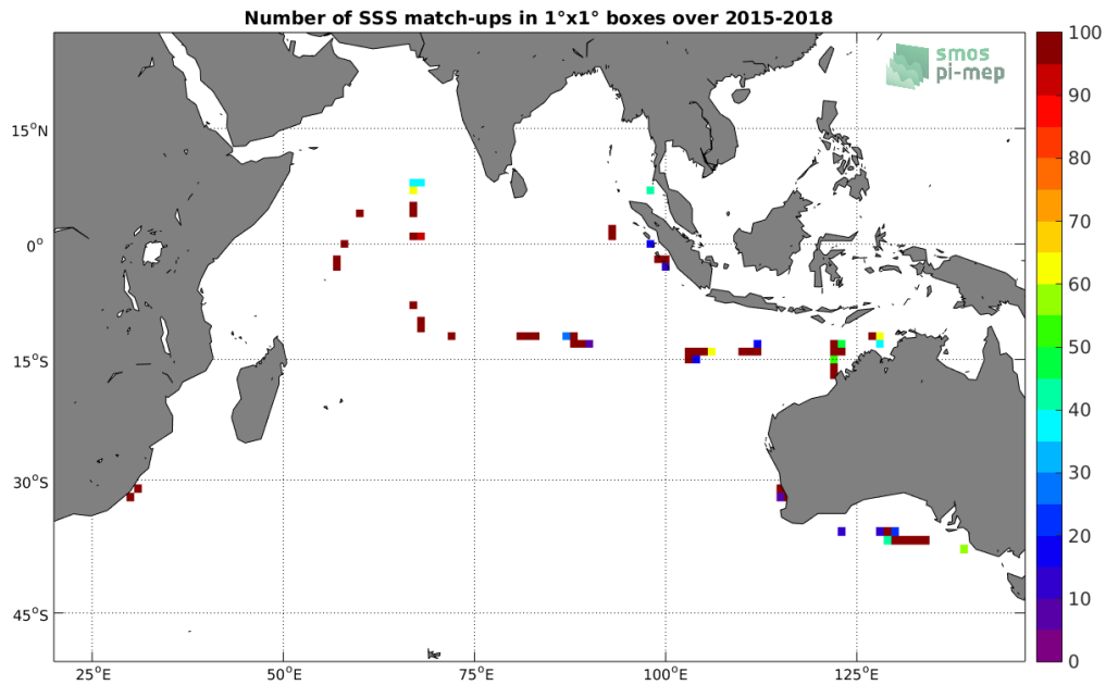
Figure 4: Number of SSS match-ups between TSG-SAMOS SSS and the SMOS-L2-DPGS-v662 SSS product for the Indian Ocean Pi-MEP region over 1^\circ \times 1^\circ boxes and for the full satellite product period.
