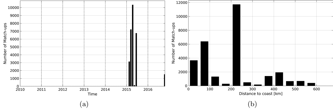
Figure 1: Number of match-ups between TSG-SAMOS and SMOS-L2-DPGS-v662 SSS as a function of time (a) and as function of the distance to coast (b) over the Indian Ocean Pi-MEP region and for the full satellite product period.
