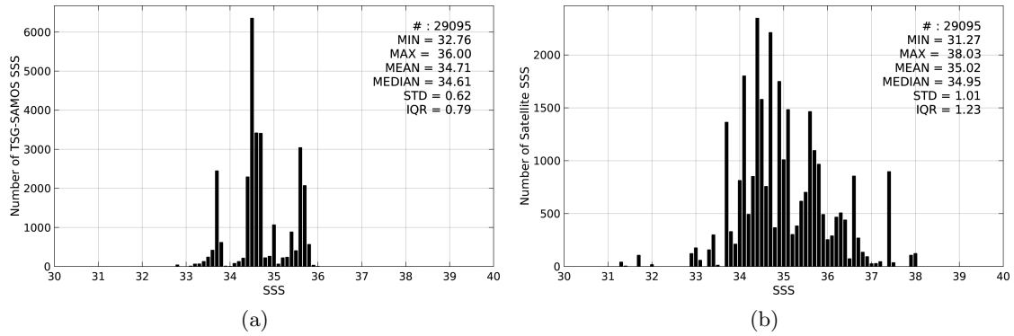
Figure 2: Histograms of SSS from TSG-SAMOS (a) and SMOS-L2-DPGS-v662 (b) considering all match-up pairs per bins of 0.1 over the Indian Ocean Pi-MEP region and for the full satellite product period.
