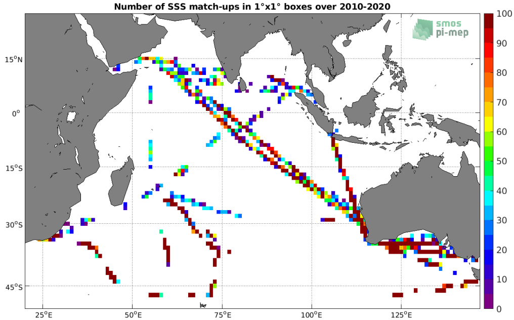
Figure 4: Number of SSS match-ups between TSG (LEGOS-DM) SSS and the SMOS SSS L2 v662 (ESA) SSS product for the Indian Ocean Pi-MEP region over 1^\circ \times 1^\circ boxes and for the full satellite product period.
