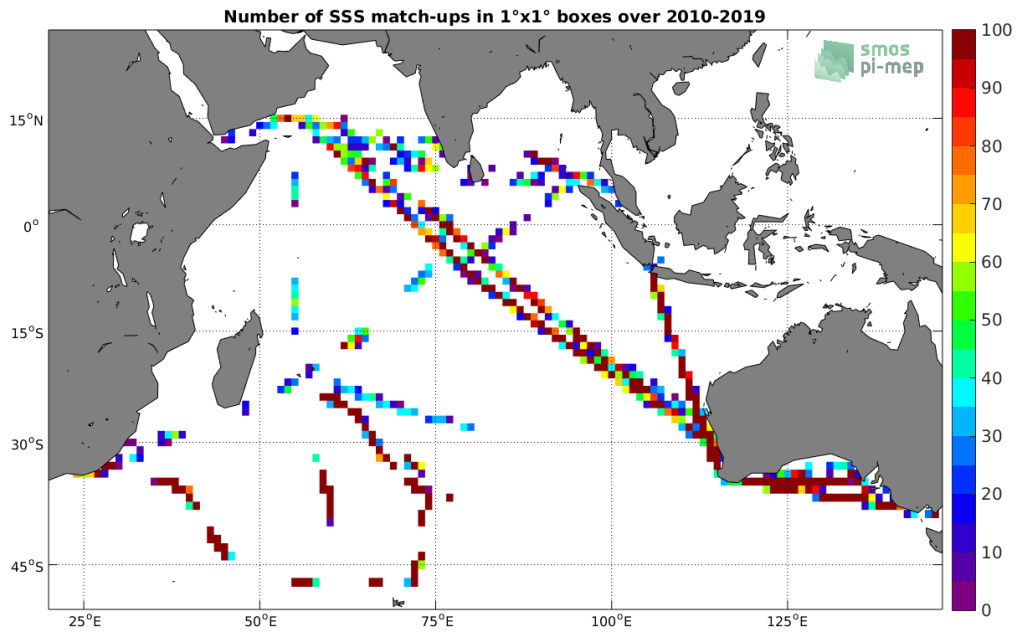
Figure 4: Number of SSS match-ups between TSG (LEGOS-DM) SSS and the SMOS SSS L2 v662 (ESA) SSS product for the Indian Ocean Pi-MEP region over 1°x1° boxes and for the full satellite product period.
