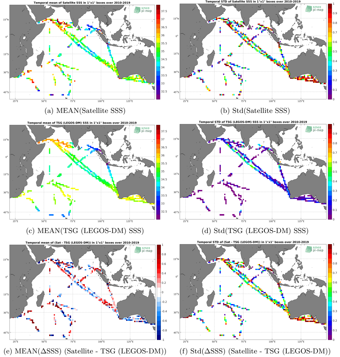
Figure 6: Temporal mean (left) and Std (right) of SSS from SMOS SSS L2 v662 (ESA) (top), TSG (LEGOS-DM) (middle), and of \Delta SSS (Satellite - TSG (LEGOS-DM)). Only match-up pairs are used to generate these maps.
