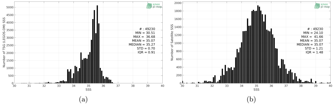
Figure 2: Histograms of SSS from TSG (LEGOS-DM) (a) and SMOS SSS L2 v662 (ESA) (b) considering all match-up pairs per bins of 0.1 over the Indian Ocean Pi-MEP region and for the full satellite product period.
