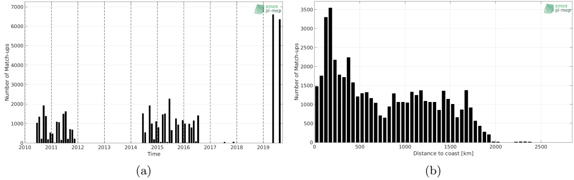
Figure 1: Number of match-ups between TSG (LEGOS-DM) and SMOS SSS L2 v662 (ESA) SSS as a function of time (a) and as function of the distance to coast (b) over the Indian Ocean Pi-MEP region and for the full satellite product period.
