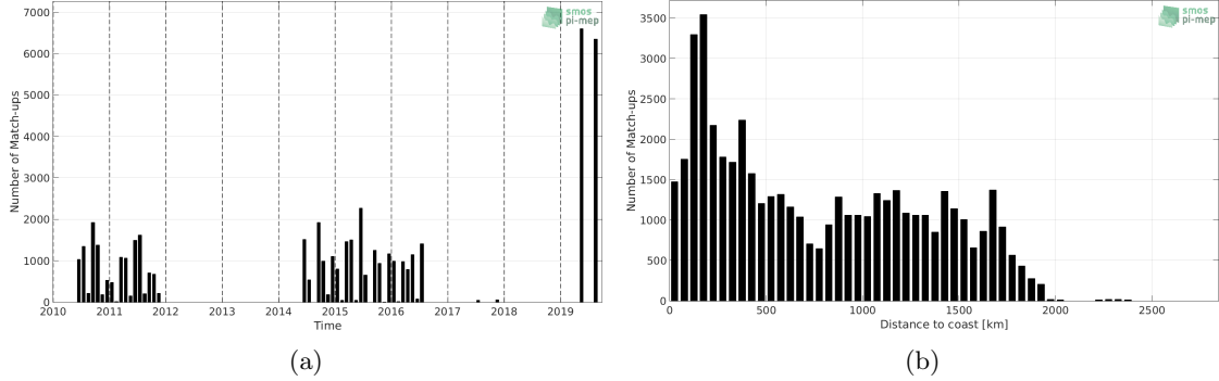
Figure 1: Number of match-ups between TSG-LEGOS-DM and SMOS L2 v662 (ESA) SSS as a function of time (a) and as function of the distance to coast (b) over the Indian Ocean Pi-MEP region and for the full satellite product period.
