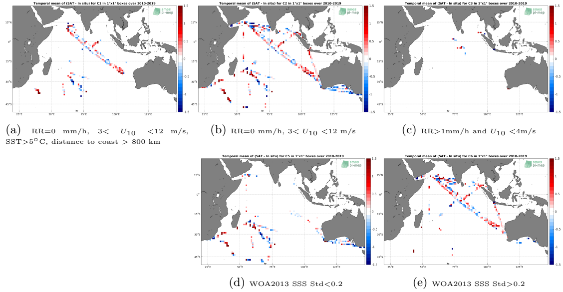
Figure 12: Temporal mean gridded over spatial boxes of size 1^\circ \times 1^\circ of \Delta SSS (SMOS L2 v662 (ESA) - TSG-LEGOS-DM) for 5 different subdatasets corresponding to: RR=0 mm/h, 3 < U_{10} < 12 m/s, SST > 5^\circ C , distance to coast > 800 km (a), RR=0 mm/h, 3 < U_{10} < 12 m/s (b), RR > 1 mm/h and U_{10} < 4 m/s (c), WOA2013 SSS Std < 0.2 (d), WOA2013 SSS Std > 0.2 (e).
