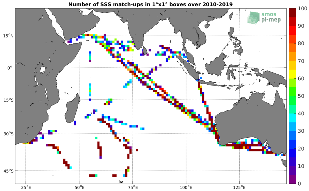
Figure 4: Number of SSS match-ups between TSG-LEGOS-DM SSS and the SMOS L2 v662 (ESA) SSS product for the Indian Ocean Pi-MEP region over 1°x1° boxes and for the full satellite product period.
