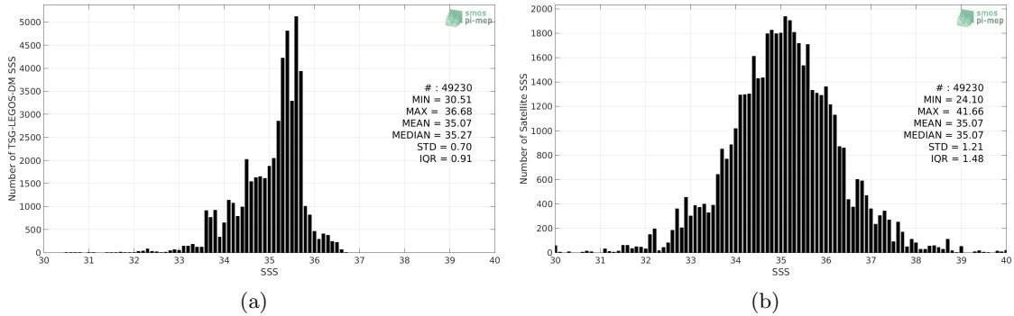
Figure 2: Histograms of SSS from TSG-LEGOS-DM (a) and SMOS L2 v662 (ESA) (b) considering all match-up pairs per bins of 0.1 over the Indian Ocean Pi-MEP region and for the full satellite product period.
