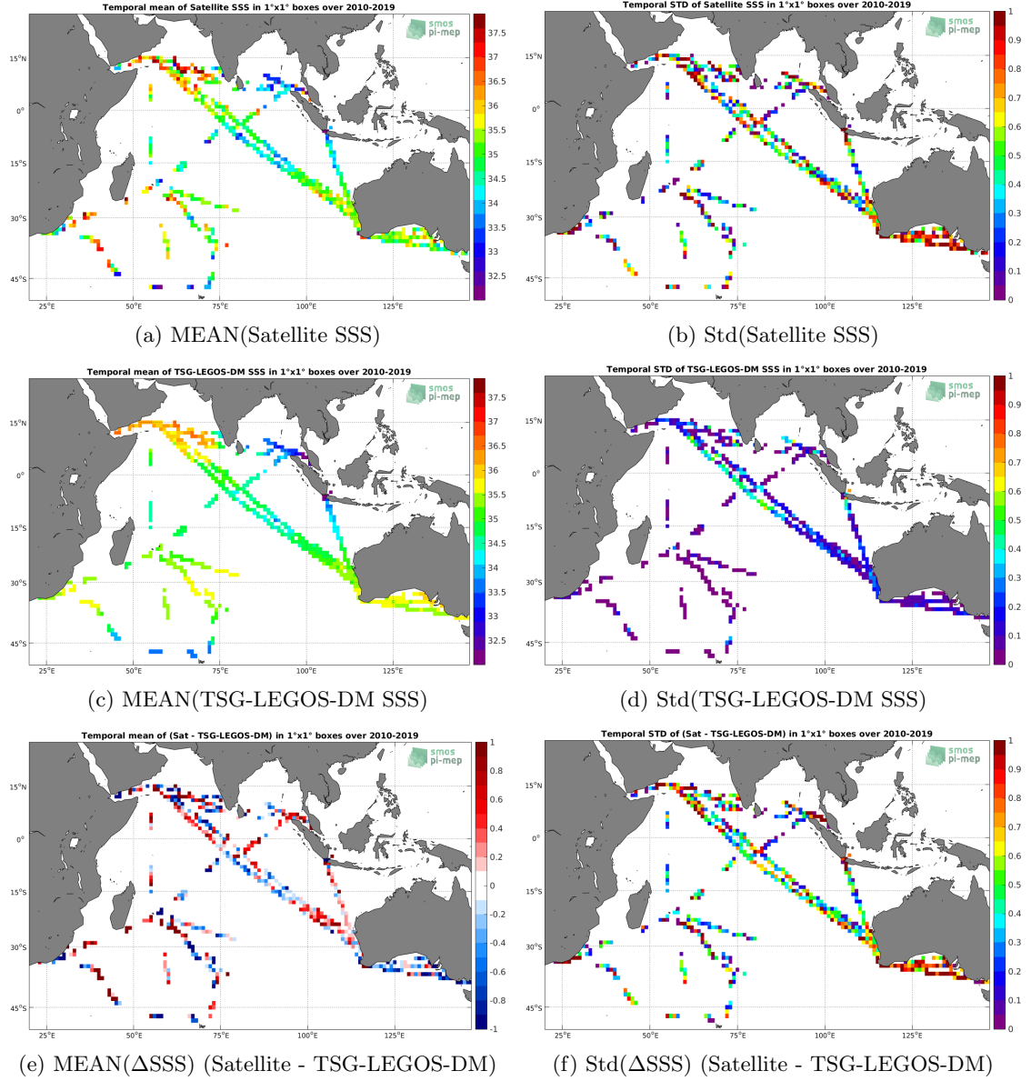
Figure 6: Temporal mean (left) and Std (right) of SSS from SMOS L2 v662 (ESA) (top), TSG-LEGOS-DM (middle), and of \Delta SSS (Satellite - TSG-LEGOS-DM). Only match-up pairs are used to generate these maps.
