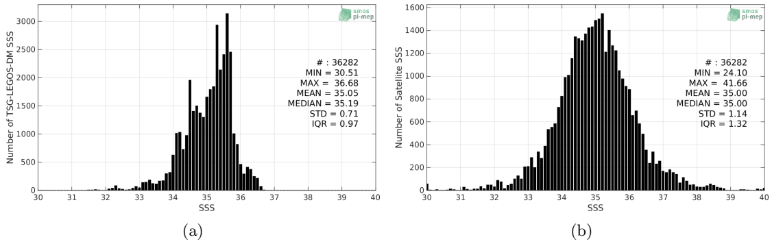
Figure 2: Histograms of SSS from TSG-LEGOS-DM (a) and SMOS-L2-DPGS-v662 (b) considering all match-up pairs per bins of 0.1 over the Indian Ocean Pi-MEP region and for the full satellite product period.
