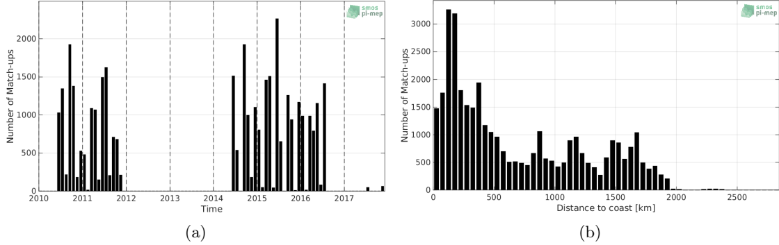
Figure 1: Number of match-ups between TSG-LEGOS-DM and SMOS-L2-DPGS-v662 SSS as a function of time (a) and as function of the distance to coast (b) over the Indian Ocean Pi-MEP region and for the full satellite product period.
