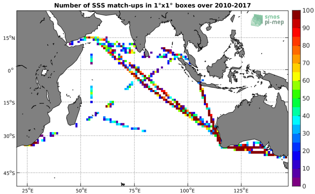
Figure 4: Number of SSS match-ups between TSG-LEGOS-DM SSS and the SMOS-L2-DPGS-v662 SSS product for the Indian Ocean Pi-MEP region over 1°x1° boxes and for the full satellite product period.
