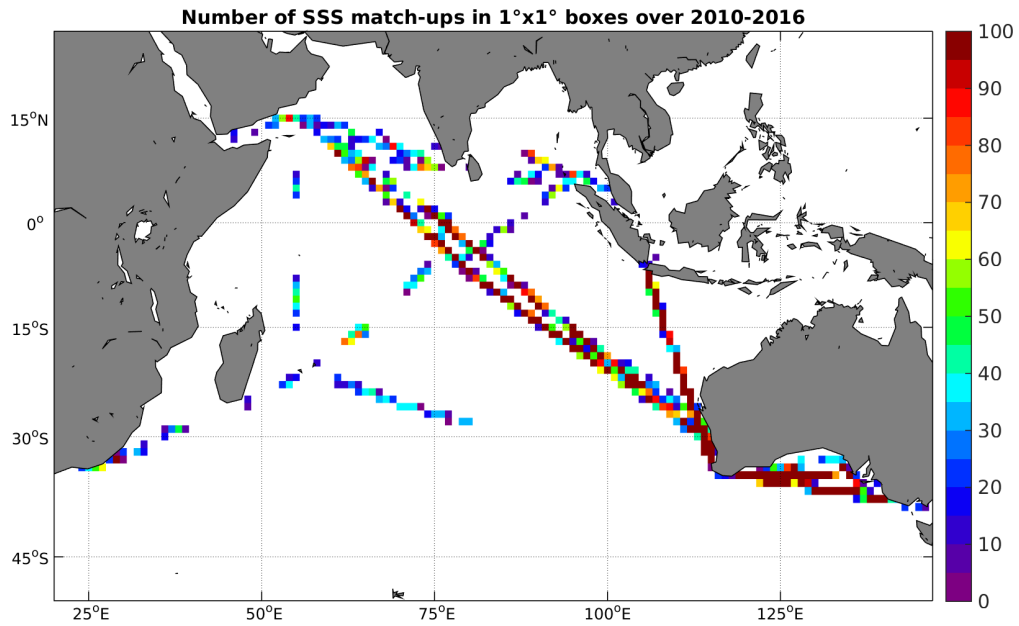
Figure 4: Number of SSS match-ups between TSG-LEGOS-DM SSS and the SMOS-L2-DPGS-v662 SSS product for the Indian Ocean Pi-MEP region over 1^\circ \times 1^\circ boxes and for the full satellite product period.
