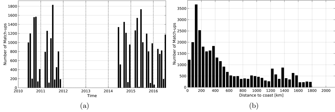
Figure 1: Number of match-ups between TSG-LEGOS-DM and SMOS-L2-DPGS-v662 SSS as a function of time (a) and as function of the distance to coast (b) over the Indian Ocean Pi-MEP region and for the full satellite product period.
