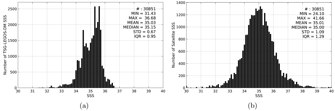
Figure 2: Histograms of SSS from TSG-LEGOS-DM (a) and SMOS-L2-DPGS-v662 (b) considering all match-up pairs per bins of 0.1 over the Indian Ocean Pi-MEP region and for the full satellite product period.
