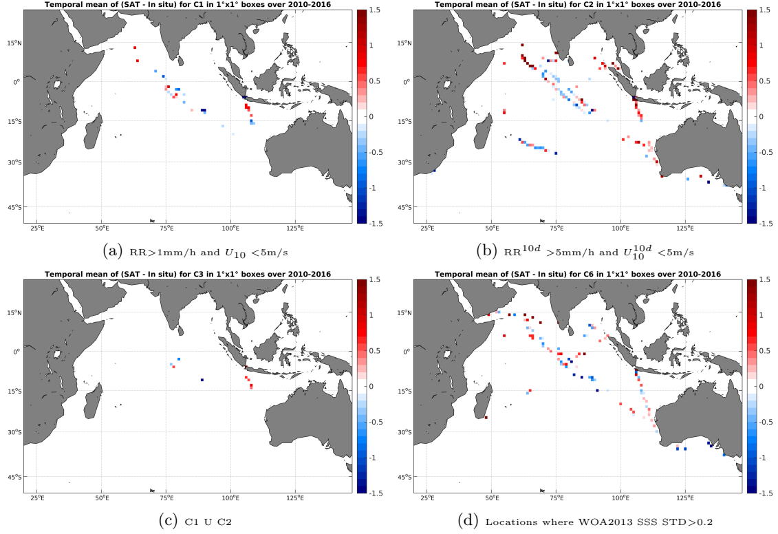
Figure 12: Temporal mean gridded over spatial boxes of size 1^\circ \times 1^\circ of \Delta SSS (SMOS-L2-DPGS-v662 - TSG-LEGOS-DM) for 4 different subdatasets corresponding to: RR > 1mm/h and U_{10} < 5 m/s (a), RR^{10d} > 5 mm/h and U_{10}^{10d} < 5 m/s (b), C1 U C2 (c), Locations where WOA2013 SSS STD > 0.2 (d).
