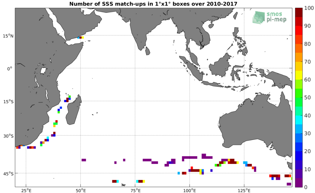
Figure 4: Number of SSS match-ups between TSG (GOSUD-Sailing-ship) SSS and the SMOS SSS L2 v662 (ESA) SSS product for the Indian Ocean Pi-MEP region over 1^\circ \times 1^\circ boxes and for the full satellite product period.
