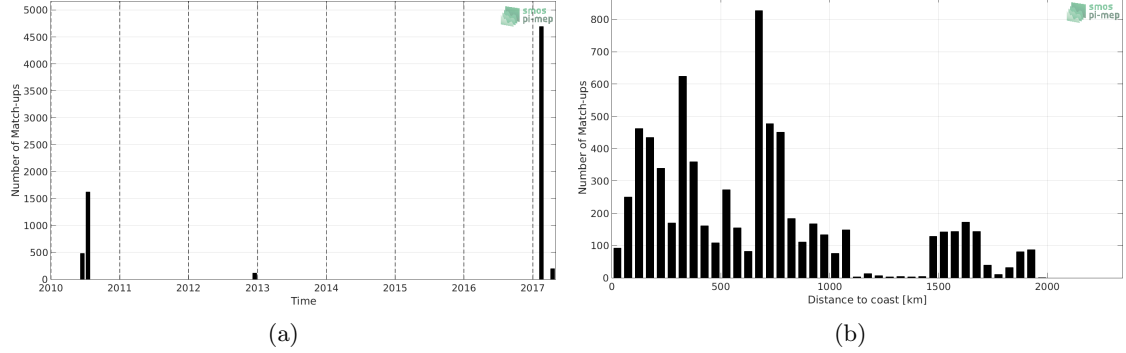
Figure 1: Number of match-ups between TSG (GOSUD-Sailing-ship) and SMOS SSS L2 v662 (ESA) SSS as a function of time (a) and as function of the distance to coast (b) over the Indian Ocean Pi-MEP region and for the full satellite product period.
