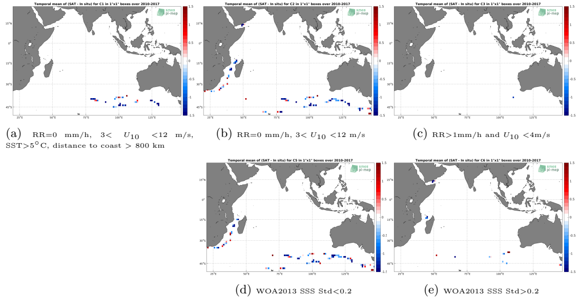
Figure 12: Temporal mean gridded over spatial boxes of size 1^\circ \times 1^\circ of \Delta SSS (SMOS SSS L2 v662 (ESA) - TSG (GOSUD-Sailing-ship)) for 5 different subdatasets corresponding to:RR=0 mm/h, 3 < U_{10} < 12 m/s, SST >5^\circ C, distance to coast > 800 km (a), RR=0 mm/h, 3 < U_{10} < 12 m/s (b), RR >1 mm/h and U_{10} < 4 m/s (c), WOA2013 SSS Std <0.2 (d), WOA2013 SSS Std >0.2 (e).
