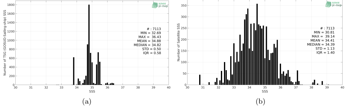
Figure 2: Histograms of SSS from TSG (GOSUD-Sailing-ship) (a) and SMOS SSS L2 v662 (ESA) (b) considering all match-up pairs per bins of 0.1 over the Indian Ocean Pi-MEP region and for the full satellite product period.
