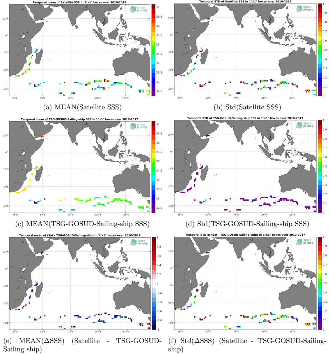
Figure 6: Temporal mean (left) and Std (right) of SSS from SMOS L2 v662 (ESA) (top), TSG-GOSUD-Sailing-ship (middle), and of \Delta SSS (Satellite - TSG-GOSUD-Sailing-ship). Only match-up pairs are used to generate these maps.
