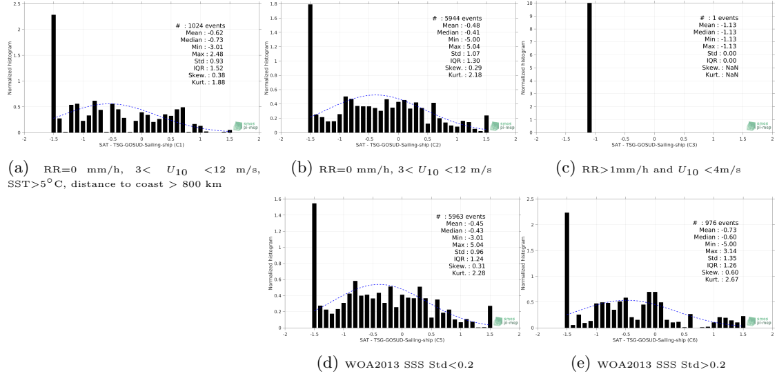
Figure 13: Normalized histogram of \Delta SSS (SMOS L2 v662 (ESA) - TSG-GOSUD-Sailing-ship) for 5 different subdatasets corresponding to: RR=0 mm/h, 3 < U_{10} < 12 m/s, SST > 5^\circ C , distance to coast > 800 km (a), RR=0 mm/h, 3 < U_{10} < 12 m/s (b), RR > 1 mm/h and U_{10} < 4 m/s (c), WOA2013 SSS Std < 0.2 (d), WOA2013 SSS Std > 0.2 (e).
