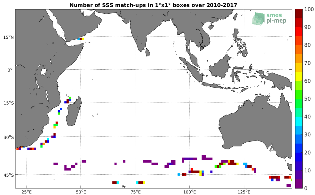
Figure 4: Number of SSS match-ups between TSG-GOSUD-Sailing-ship SSS and the SMOS L2 v662 (ESA) SSS product for the Indian Ocean Pi-MEP region over 1°x1° boxes and for the full satellite product period.
