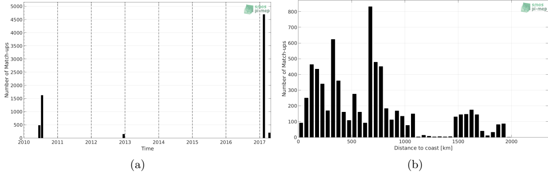
Figure 1: Number of match-ups between TSG-GOSUD-Sailing-ship and SMOS L2 v662 (ESA) SSS as a function of time (a) and as function of the distance to coast (b) over the Indian Ocean Pi-MEP region and for the full satellite product period.
