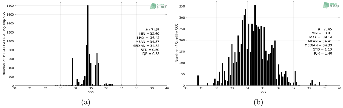
Figure 2: Histograms of SSS from TSG-GOSUD-Sailing-ship (a) and SMOS L2 v662 (ESA) (b) considering all match-up pairs per bins of 0.1 over the Indian Ocean Pi-MEP region and for the full satellite product period.
