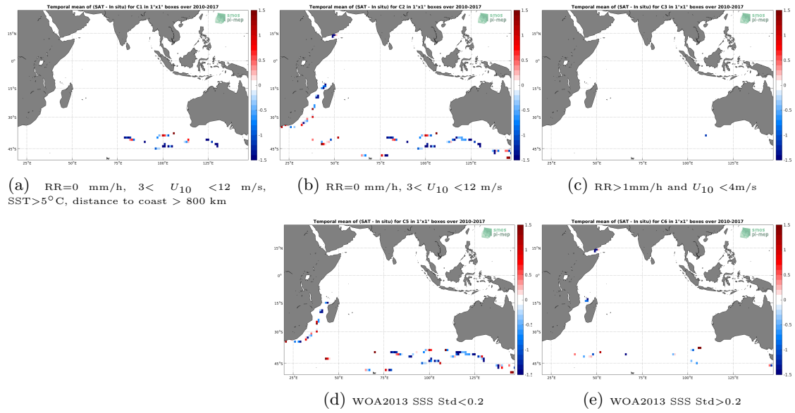
Figure 12: Temporal mean gridded over spatial boxes of size 1^\circ \times 1^\circ of \Delta SSS (SMOS L2 v662 (ESA) - TSG-GOSUD-Sailing-ship) for 5 different subdatasets corresponding to:RR=0 mm/h, 3 < U_{10} < 12 m/s, SST >5^\circ\text{C} , distance to coast > 800 km (a), RR=0 mm/h, 3 < U_{10} < 12 m/s (b), RR >1 mm/h and U_{10} < 4 m/s (c), WOA2013 SSS Std <0.2 (d), WOA2013 SSS Std >0.2 (e).
