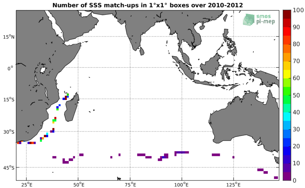
Figure 4: Number of SSS match-ups between TSG-GOSUD-Sailing-ship SSS and the SMOS-L2-DPGS-v662 SSS product for the Indian Ocean Pi-MEP region over 1°x1° boxes and for the full satellite product period.
