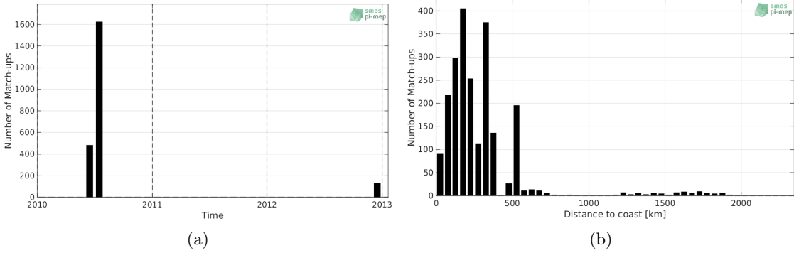
Figure 1: Number of match-ups between TSG-GOSUD-Sailing-ship and SMOS-L2-DPGS-v662 SSS as a function of time (a) and as function of the distance to coast (b) over the Indian Ocean Pi-MEP region and for the full satellite product period.
