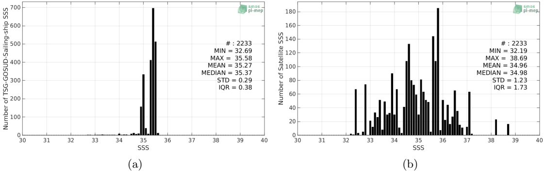
Figure 2: Histograms of SSS from TSG-GOSUD-Sailing-ship (a) and SMOS-L2-DPGS-v662 (b) considering all match-up pairs per bins of 0.1 over the Indian Ocean Pi-MEP region and for the full satellite product period.
