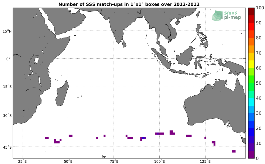
Figure 4: Number of SSS match-ups between TSG-GOSUD-Sailing-ship SSS and the SMOS-L2-DPGS-v662 SSS product for the Indian Ocean Pi-MEP region over 1^\circ \times 1^\circ boxes and for the full satellite product period.
