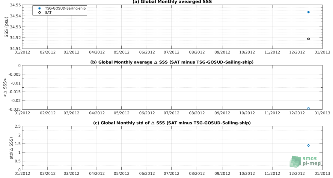
Figure 7: Time series of the monthly averaged mean SSS (top), mean \Delta SSS (Satellite - TSG-GOSUD-Sailing-ship) and STD of \Delta SSS (Satellite - TSG-GOSUD-Sailing-ship) over the Indian Ocean Pi-MEP region considering all match-ups collected by the Pi-MEP platform.
