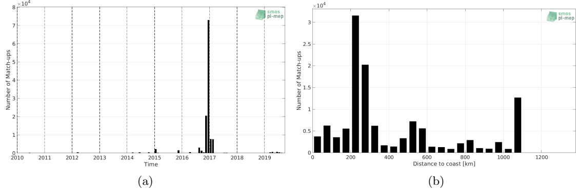
Figure 1: Number of match-ups between TSG (GOSUD-Research-vessel) and SMOS SSS L2 v662 (ESA) SSS as a function of time (a) and as function of the distance to coast (b) over the Indian Ocean Pi-MEP region and for the full satellite product period.
