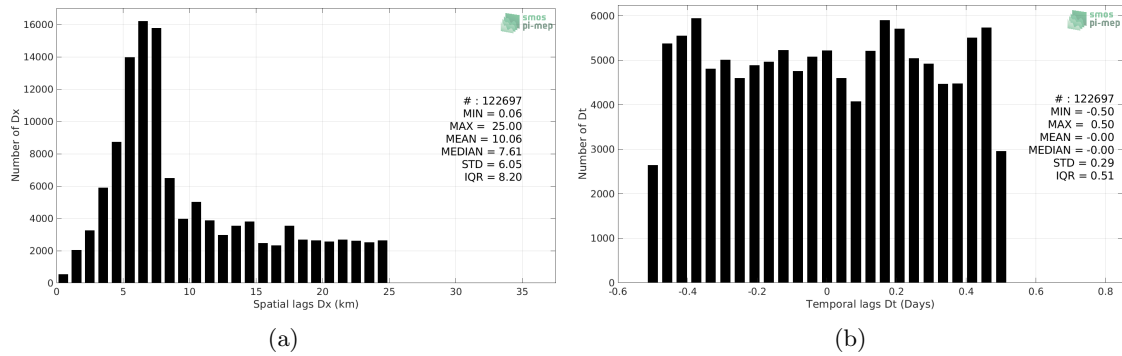
Figure 5: Histograms of the spatial (a) and temporal (b) lags between the location/time of the TSG (GOSUD-Research-vessel) measurement and the date of the corresponding SMOS SSS L2 v662 (ESA) SSS pixel.
