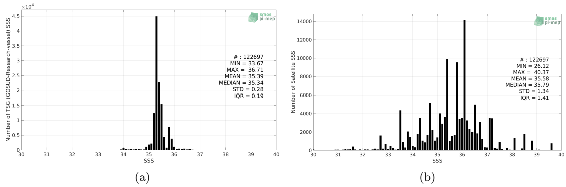
Figure 2: Histograms of SSS from TSG (GOSUD-Research-vessel) (a) and SMOS SSS L2 v662 (ESA) (b) considering all match-up pairs per bins of 0.1 over the Indian Ocean Pi-MEP region and for the full satellite product period.
