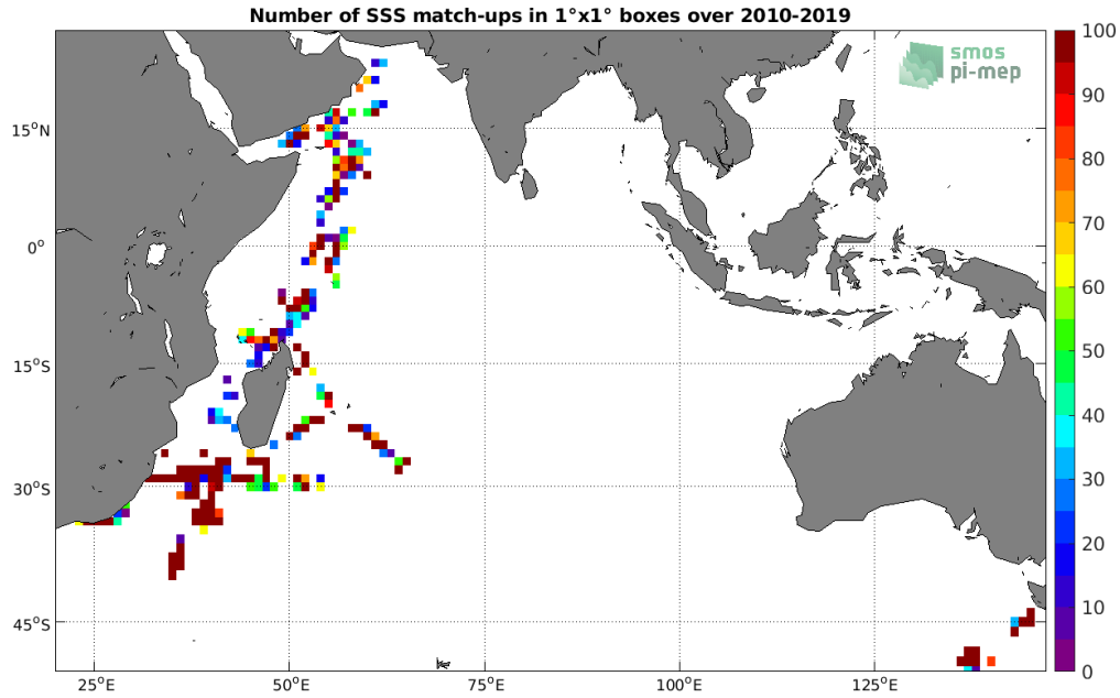
Figure 4: Number of SSS match-ups between TSG (GOSUD-Research-vessel) SSS and the SMOS SSS L2 v662 (ESA) SSS product for the Indian Ocean Pi-MEP region over 1^\circ \times 1^\circ boxes and for the full satellite product period.
