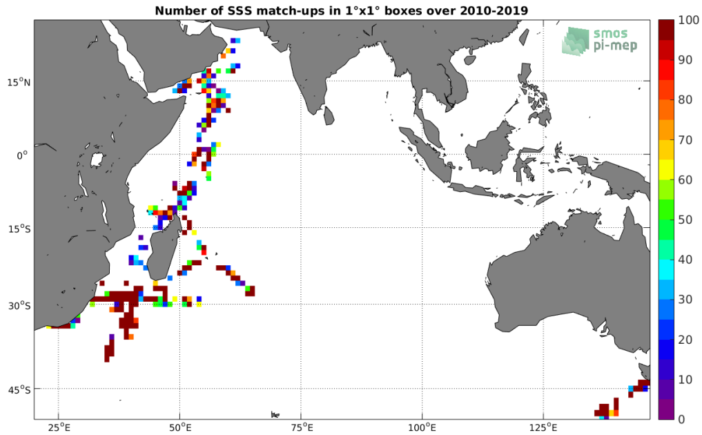
Figure 4: Number of SSS match-ups between TSG (GOSUD-Research-vessel) SSS and the SMOS SSS L2 v662 (ESA) SSS product for the Indian Ocean Pi-MEP region over 1°x1° boxes and for the full satellite product period.
