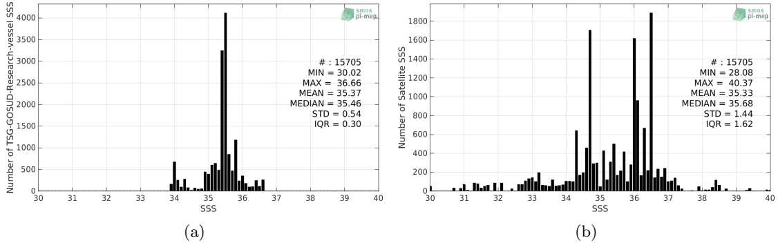
Figure 2: Histograms of SSS from TSG-GOSUD-Research-vessel (a) and SMOS-L2-DPGS-v662 (b) considering all match-up pairs per bins of 0.1 over the Indian Ocean Pi-MEP region and for the full satellite product period.
