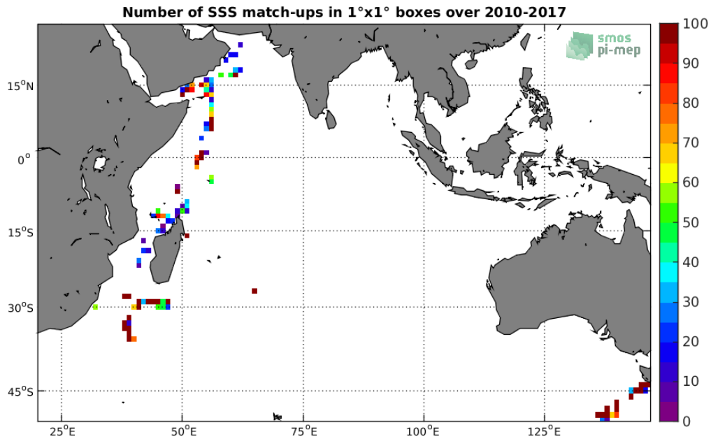
Figure 4: Number of SSS match-ups between TSG-GOSUD-Research-vessel SSS and the SMOS-L2-DPGS-v662 SSS product for the Indian Ocean Pi-MEP region over 1°x1° boxes and for the full satellite product period.
