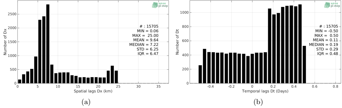
Figure 5: Histograms of the spatial (a) and temporal (b) lags between the time of the TSG-GOSUD-Research-vessel measurements and the date of the corresponding SMOS-L2-DPGS-v662 SSS product.
