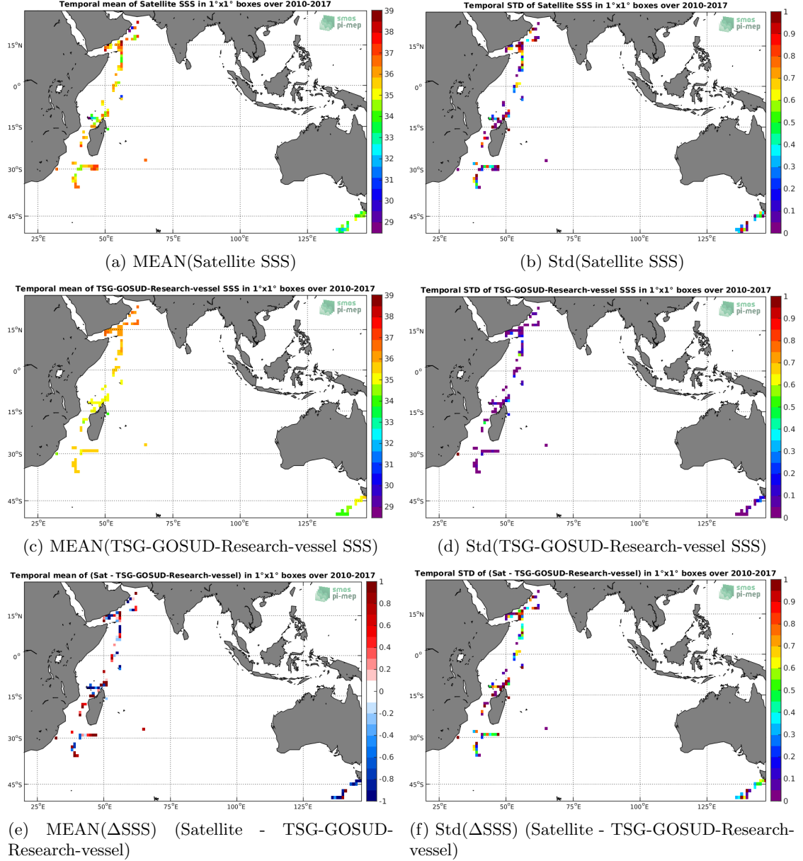
Figure 6: Temporal mean (left) and Std (right) of SSS from SMOS-L2-DPGS-v662 (top), TSG-GOSUD-Research-vessel (middle), and of \Delta SSS (Satellite - TSG-GOSUD-Research-vessel). Only match-up pairs are used to generate these maps.
