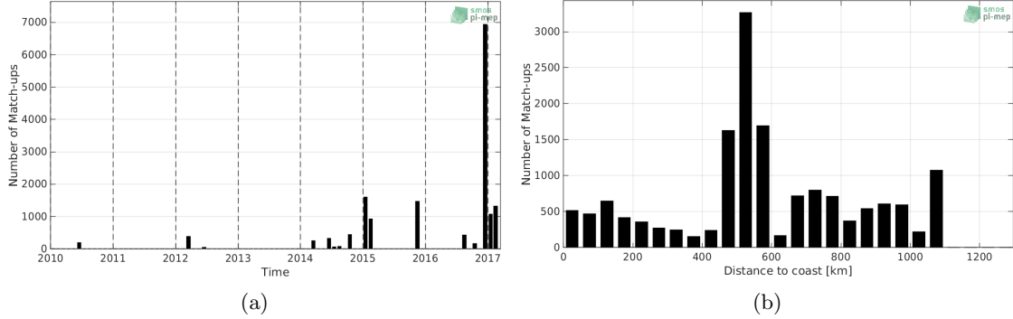
Figure 1: Number of match-ups between TSG-GOSUD-Research-vessel and SMOS-L2-DPGS-v662 SSS as a function of time (a) and as function of the distance to coast (b) over the Indian Ocean Pi-MEP region and for the full satellite product period.
