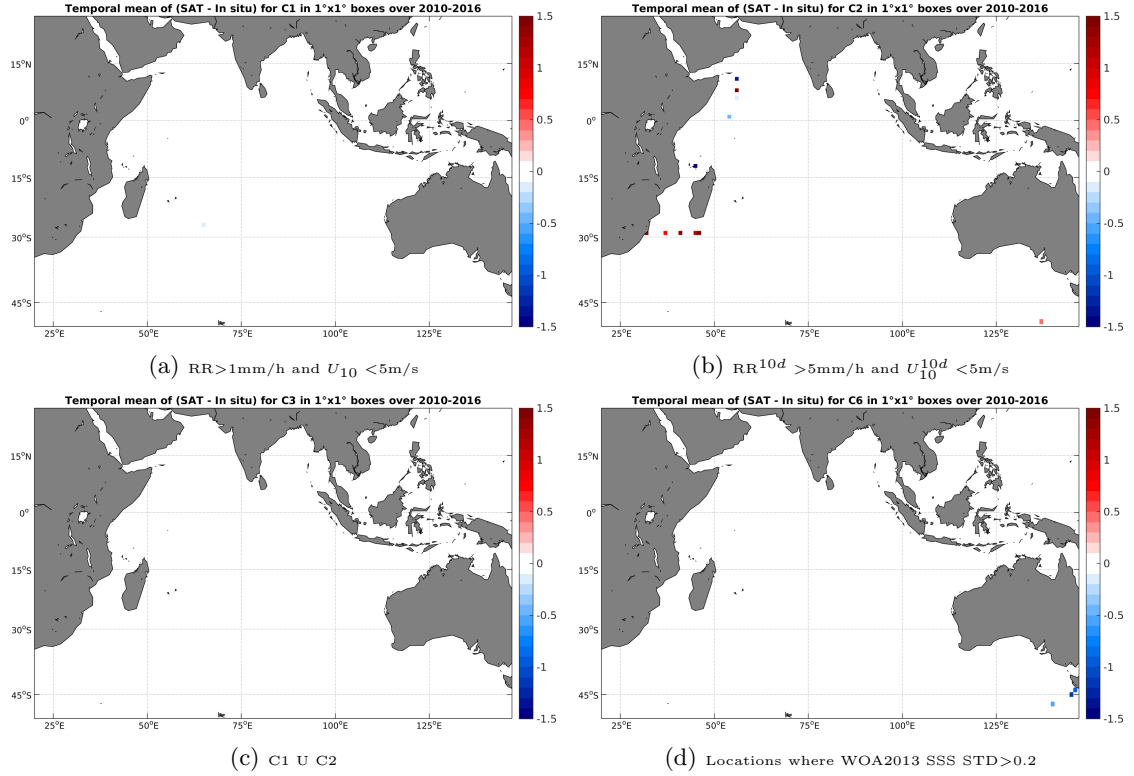
Figure 12: Temporal mean gridded over spatial boxes of size 1^\circ \times 1^\circ of \Delta SSS (SMOS-L2-DPGS-v662 - TSG-GOSUD-Research-vessel) for 4 different subdatasets corresponding to: RR > 1\text{mm/h} and U_{10} < 5\text{m/s} (a), RR^{10d} > 5\text{mm/h} and U_{10}^{10d} < 5\text{m/s} (b), C1 U C2 (c), Locations where WOA2013 SSS STD > 0.2 (d).
