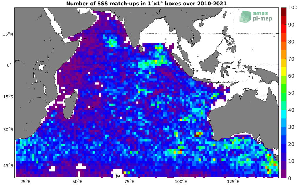
Figure 4: Number of SSS match-ups between Argo SSS and the SMOS SSS L2 v662 (ESA) SSS product for the Indian Ocean Pi-MEP region over 1^\circ \times 1^\circ boxes and for the full satellite product period.
