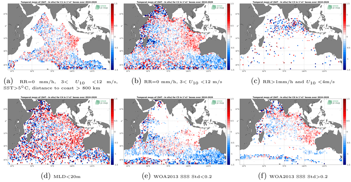
Figure 12: Temporal mean gridded over spatial boxes of size 1^\circ \times 1^\circ of \Delta SSS (SMOS L2 v662 (ESA) - Argo) for 6 different subdatasets corresponding to: RR=0 mm/h, 3 < U_{10} < 12 m/s, SST >5^\circ C, distance to coast > 800 km (a), RR=0 mm/h, 3 < U_{10} < 12 m/s (b), RR >1 mm/h and U_{10} < 4 m/s (c), MLD <20 m (d), WOA2013 SSS Std <0.2 (e), WOA2013 SSS Std >0.2 (f).
