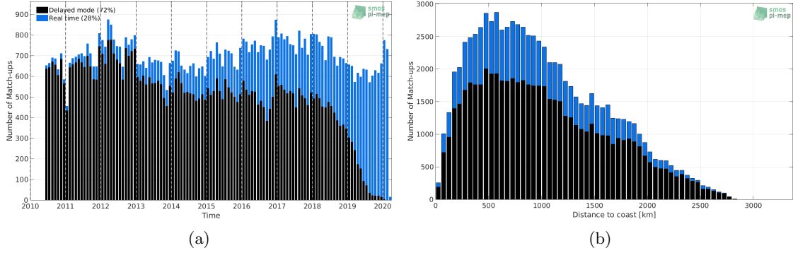
Figure 1: Number of match-ups between Argo and SMOS L2 v662 (ESA) SSS as a function of time (a) and as function of the distance to coast (b) over the Indian Ocean Pi-MEP region and for the full satellite product period.
