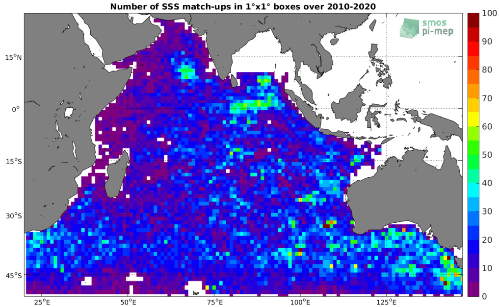
Figure 4: Number of SSS match-ups between Argo SSS and the SMOS L2 v662 (ESA) SSS product for the Indian Ocean Pi-MEP region over 1^\circ \times 1^\circ boxes and for the full satellite product period.
