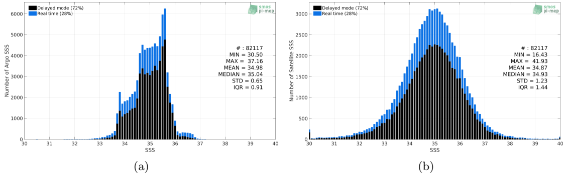
Figure 2: Histograms of SSS from Argo (a) and SMOS L2 v662 (ESA) (b) considering all match-up pairs per bins of 0.1 over the Indian Ocean Pi-MEP region and for the full satellite product period.
