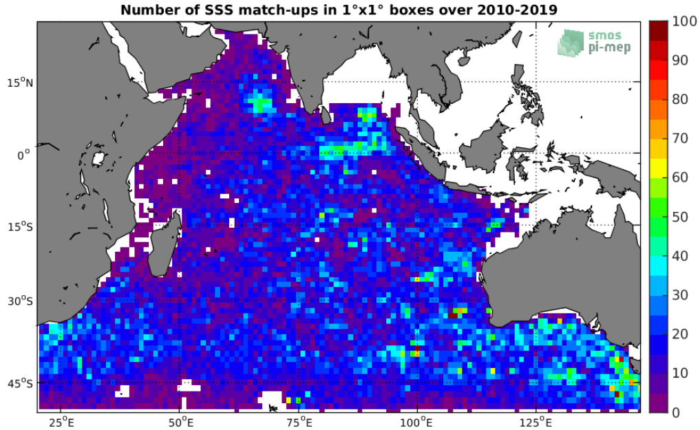
Figure 4: Number of SSS match-ups between Argo SSS and the SMOS-L2-DPGS-v662 SSS product for the Indian Ocean Pi-MEP region over 1°x1° boxes and for the full satellite product period.
