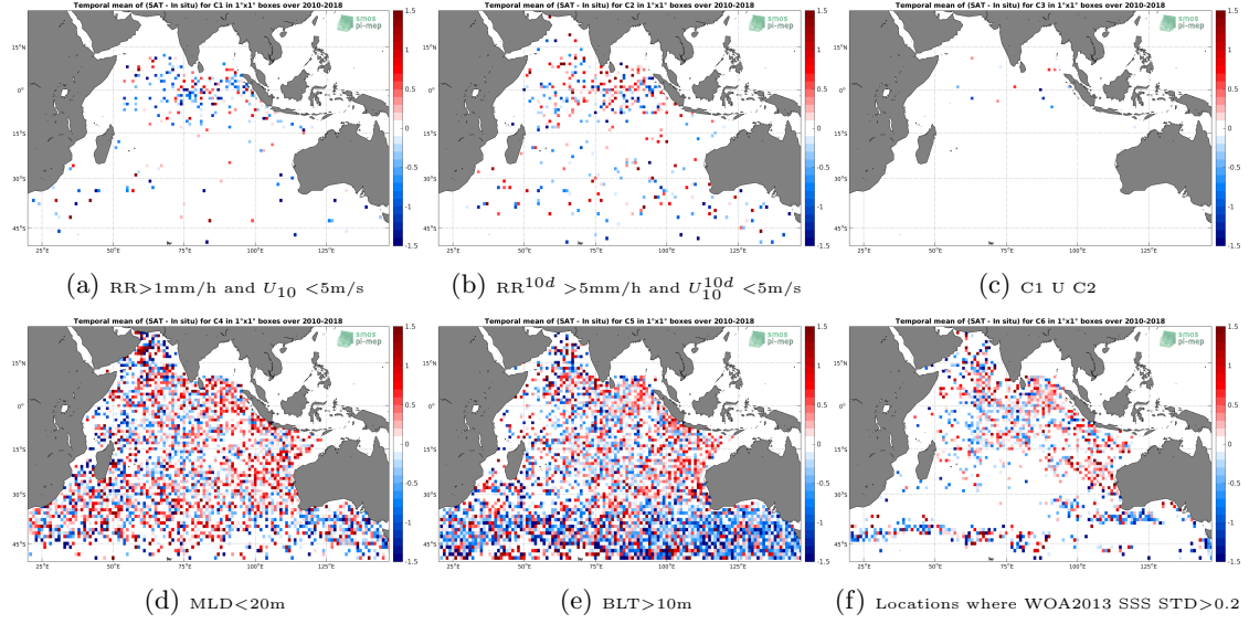
Figure 12: Temporal mean gridded over spatial boxes of size 1^\circ \times 1^\circ of \Delta\text{SSS} (SMOS-L2-DPGS-v662 - Argo) for 6 different subdatasets corresponding to: \text{RR} > 1\text{mm/h} and U_{10} < 5\text{m/s} (a), \text{RR}^{10d} > 5\text{mm/h} and U_{10}^{10d} < 5\text{m/s} (b), C1 U C2 (c), \text{MLD} < 20\text{m} (d), \text{BLT} > 10\text{m} (e), Locations where WOA2013 SSS STD > 0.2 (f).
