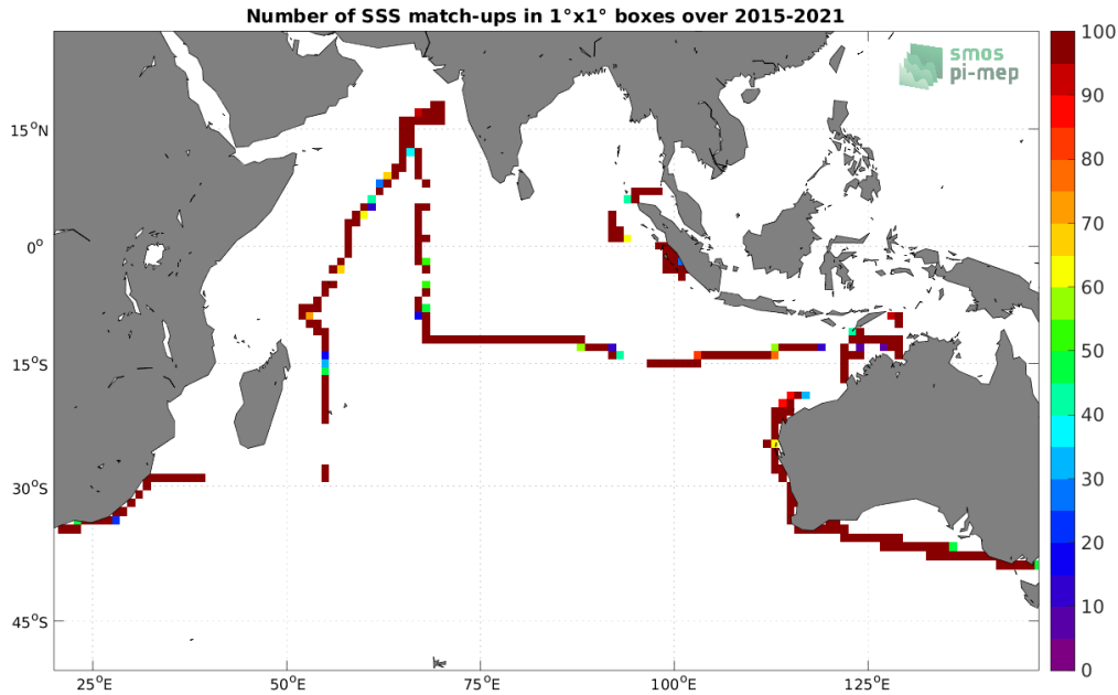
Figure 4: Number of SSS match-ups between TSG (SAMOS) SSS and the SMAP SSS L4 OI v1 - 7 Days (IPRC) SSS product for the Indian Ocean Pi-MEP region over 1^\circ \times 1^\circ boxes and for the full satellite product period.
