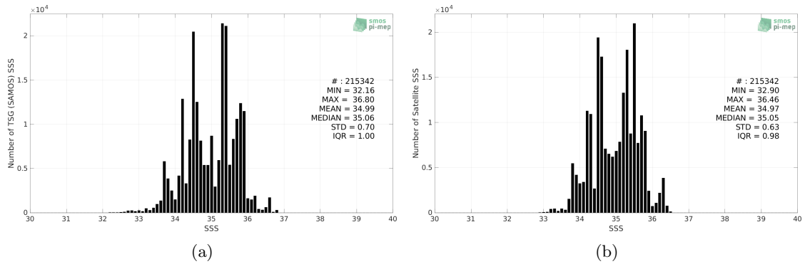
Figure 2: Histograms of SSS from TSG (SAMOS) (a) and SMAP SSS L4 OI v1 - 7 Days (IPRC) (b) considering all match-up pairs per bins of 0.1 over the Indian Ocean Pi-MEP region and for the full satellite product period.
