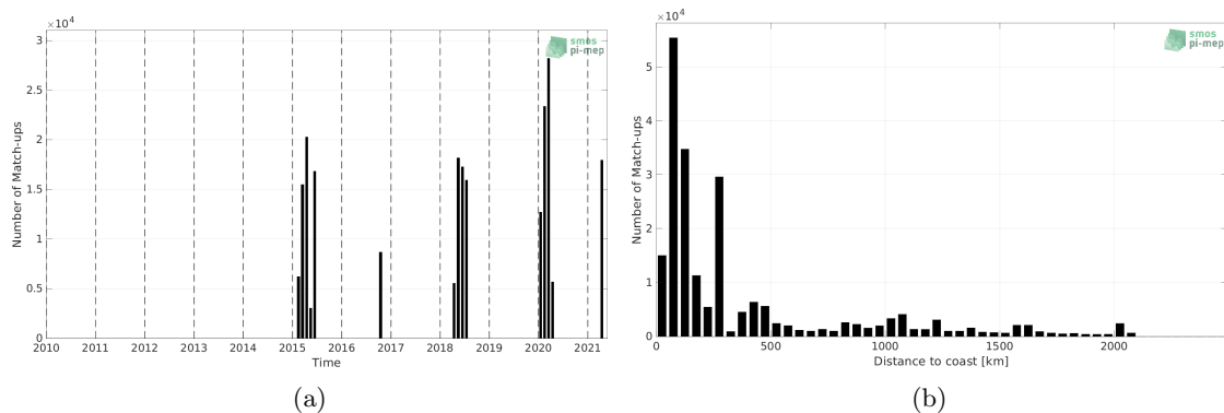
Figure 1: Number of match-ups between TSG (SAMOS) and SMAP SSS L4 OI v1 - 7 Days (IPRC) SSS as a function of time (a) and as function of the distance to coast (b) over the Indian Ocean Pi-MEP region and for the full satellite product period.
