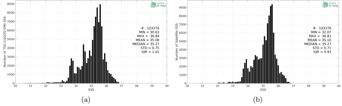
Figure 2: Histograms of SSS from TSG (LEGOS-DM) (a) and SMAP SSS L4 OI v1 - 7 Days (IPRC) (b) considering all match-up pairs per bins of 0.1 over the Indian Ocean Pi-MEP region and for the full satellite product period.
