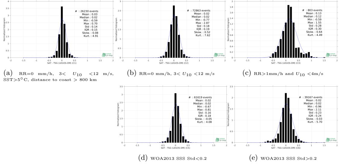
Figure 13: Normalized histogram of \Delta SSS (SMAP SSS L4 OI v1 - 7day (IPRC) - TSG (LEGOS-DM)) for 5 different subdatasets corresponding to: RR=0 mm/h, 3 < U_{10} < 12 m/s, SST>5°C, distance to coast > 800 km (a), RR=0 mm/h, 3 < U_{10} < 12 m/s (b), RR>1mm/h and U_{10} < 4 m/s (c), WOA2013 SSS Std<0.2 (d), WOA2013 SSS Std>0.2 (e).
