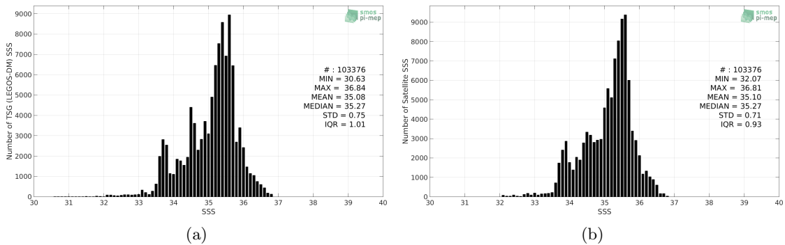
Figure 2: Histograms of SSS from TSG (LEGOS-DM) (a) and SMAP SSS L4 OI v1 - 7day (IPRC) (b) considering all match-up pairs per bins of 0.1 over the Indian Ocean Pi-MEP region and for the full satellite product period.
