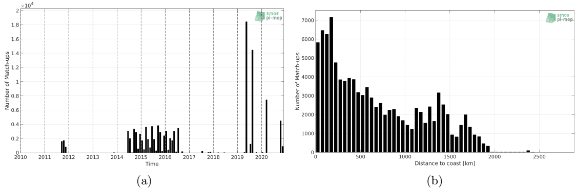
Figure 1: Number of match-ups between TSG (LEGOS-DM) and SMAP SSS L4 OI v1 - 7day (IPRC) SSS as a function of time (a) and as function of the distance to coast (b) over the Indian Ocean Pi-MEP region and for the full satellite product period.
