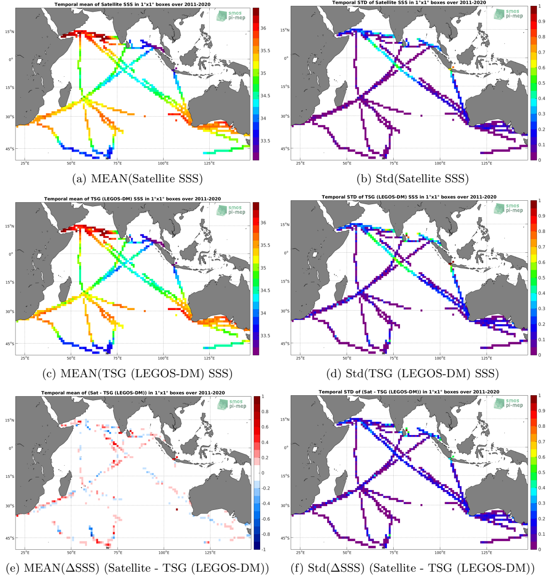
Figure 6: Temporal mean (left) and Std (right) of SSS from SMAP SSS L4 OI v1 - 7day (IPRC) (top), TSG (LEGOS-DM) (middle), and of \Delta SSS (Satellite - TSG (LEGOS-DM)). Only match-up pairs are used to generate these maps.
