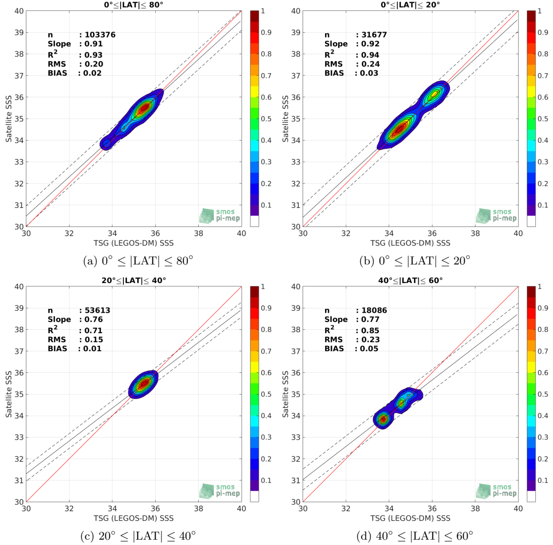
Figure 9: Contour maps of the concentration of SMAP SSS L4 OI v1 - 7day (IPRC) SSS (y-axis) versus TSG (LEGOS-DM) SSS (x-axis) at match-up pairs for different latitude bands. For each plot, the red line shows x=y . The black thin and dashed lines indicate a linear fit through the data cloud and the \pm 95\% confidence levels, respectively. The number match-up pairs n , the slope and R^2 coefficient of the linear fit, the root mean square (RMS) and the mean bias between satellite and in situ data are indicated for each latitude band in each plots.
