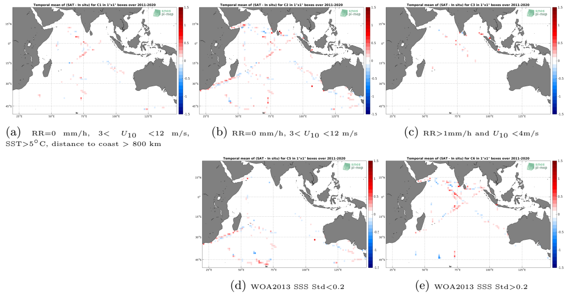
Figure 12: Temporal mean gridded over spatial boxes of size 1^\circ \times 1^\circ of \Delta SSS (SMAP SSS L4 OI v1 - 7day (IPRC) - TSG (LEGOS-DM)) for 5 different subdatasets corresponding to: RR=0 mm/h, 3 < U_{10} < 12 m/s, SST > 5^\circ C , distance to coast > 800 km (a), RR=0 mm/h, 3 < U_{10} < 12 m/s (b), RR > 1 mm/h and U_{10} < 4 m/s (c), WOA2013 SSS Std < 0.2 (d), WOA2013 SSS Std > 0.2 (e).
