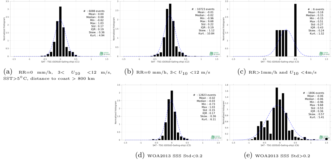
Figure 13: Normalized histogram of \Delta\text{SSS} (SMAP SSS L4 OI v1 - 7 Days (IPRC) - TSG (GOSUD-Sailing-ship)) for 5 different subdatasets corresponding to: RR=0 mm/h, 3 < U_{10} < 12 m/s, SST >5^{\circ}\text{C} , distance to coast > 800 km (a), RR=0 mm/h, 3 < U_{10} < 12 m/s (b), RR >1 mm/h and U_{10} < 4 m/s (c), WOA2013 SSS Std <0.2 (d), WOA2013 SSS Std >0.2 (e).
