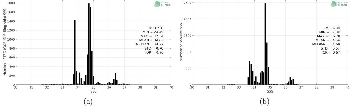
Figure 2: Histograms of SSS from TSG (GOSUD-Sailing-ship) (a) and SMAP SSS L4 OI v1 - 7 Days (IPRC) (b) considering all match-up pairs per bins of 0.1 over the Indian Ocean Pi-MEP region and for the full satellite product period.
