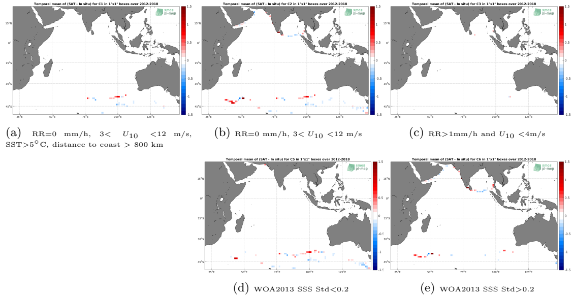
Figure 12: Temporal mean gridded over spatial boxes of size 1^\circ \times 1^\circ of \Delta SSS (SMAP SSS L4 OI v1 - 7 Days (IPRC) - TSG (GOSUD-Sailing-ship)) for 5 different subdatasets corresponding to: RR=0 mm/h, 3 < U_{10} < 12 m/s, SST > 5^\circ\text{C} , distance to coast > 800 km (a), RR=0 mm/h, 3 < U_{10} < 12 m/s (b), RR > 1 mm/h and U_{10} < 4 m/s (c), WOA2013 SSS Std < 0.2 (d), WOA2013 SSS Std > 0.2 (e).
