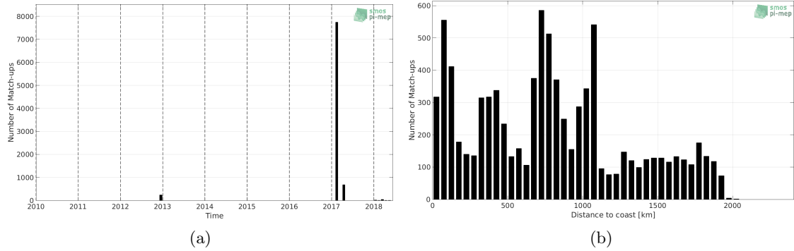
Figure 1: Number of match-ups between TSG (GOSUD-Sailing-ship) and SMAP SSS L4 OI v1 - 7 Days (IPRC) SSS as a function of time (a) and as function of the distance to coast (b) over the Indian Ocean Pi-MEP region and for the full satellite product period.
