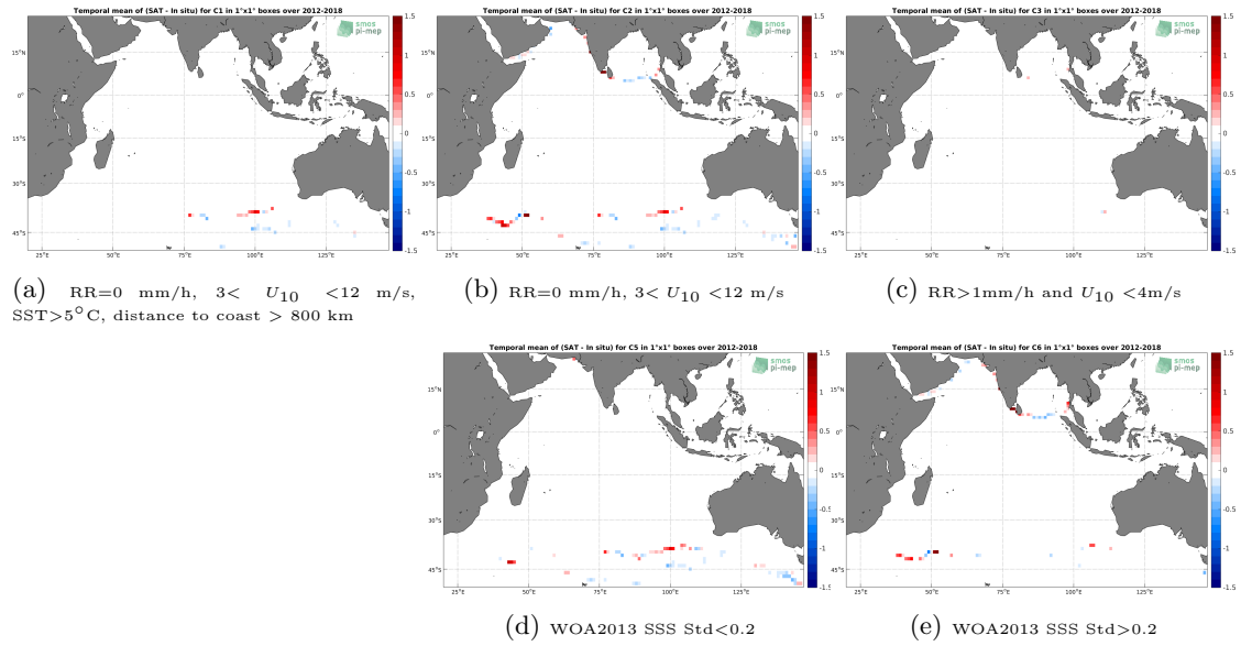
Figure 12: Temporal mean gridded over spatial boxes of size 1^\circ \times 1^\circ of \Delta SSS (SMAP SSS L4 OI v1 - 7day (IPRC) - TSG (GOSUD-Sailing-ship)) for 5 different subdatasets corresponding to: RR=0 mm/h, 3 < U_{10} < 12 m/s, SST > 5^\circ C , distance to coast > 800 km (a), RR=0 mm/h, 3 < U_{10} < 12 m/s (b), RR > 1 mm/h and U_{10} < 4 m/s (c), WOA2013 SSS Std < 0.2 (d), WOA2013 SSS Std > 0.2 (e).
