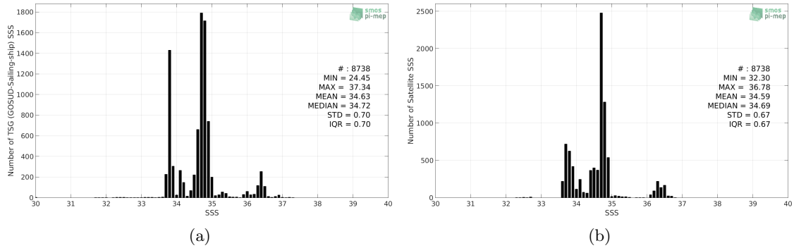
Figure 2: Histograms of SSS from TSG (GOSUD-Sailing-ship) (a) and SMAP SSS L4 OI v1 - 7day (IPRC) (b) considering all match-up pairs per bins of 0.1 over the Indian Ocean Pi-MEP region and for the full satellite product period.
