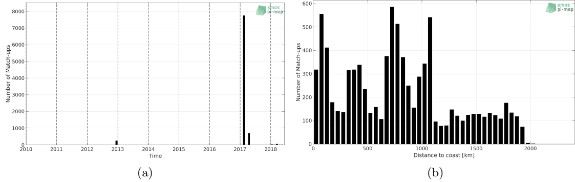
Figure 1: Number of match-ups between TSG (GOSUD-Sailing-ship) and SMAP SSS L4 OI v1 - 7day (IPRC) SSS as a function of time (a) and as function of the distance to coast (b) over the Indian Ocean Pi-MEP region and for the full satellite product period.
