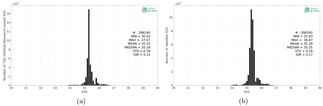
Figure 2: Histograms of SSS from TSG (GOSUD-Research-vessel) (a) and SMAP SSS L4 OI v1 - 7 Days (IPRC) (b) considering all match-up pairs per bins of 0.1 over the Indian Ocean Pi-MEP region and for the full satellite product period.
