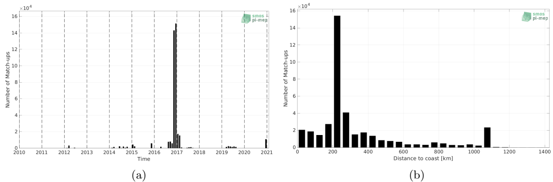
Figure 1: Number of match-ups between TSG (GOSUD-Research-vessel) and SMAP SSS L4 OI v1 - 7 Days (IPRC) SSS as a function of time (a) and as function of the distance to coast (b) over the Indian Ocean Pi-MEP region and for the full satellite product period.
