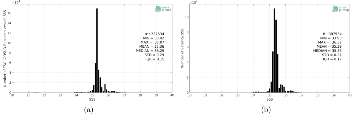
Figure 2: Histograms of SSS from TSG (GOSUD-Research-vessel) (a) and SMAP SSS L4 OI v1 - 7day (IPRC) (b) considering all match-up pairs per bins of 0.1 over the Indian Ocean Pi-MEP region and for the full satellite product period.
