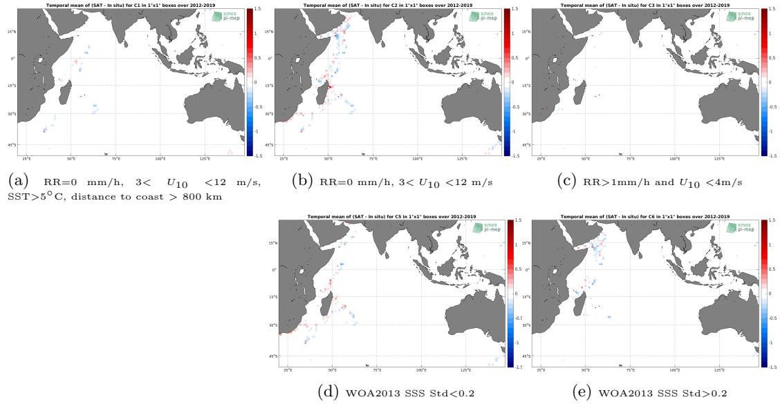
Figure 12: Temporal mean gridded over spatial boxes of size 1^\circ \times 1^\circ of \Delta SSS (SMAP SSS L4 OI v1 - 7day (IPRC) - TSG (GOSUD-Research-vessel)) for 5 different subdatasets corresponding to: RR=0 mm/h, 3 < U_{10} < 12 m/s, SST > 5^\circ C , distance to coast > 800 km (a), RR=0 mm/h, 3 < U_{10} < 12 m/s (b), RR > 1 mm/h and U_{10} < 4 m/s (c), WOA2013 SSS Std < 0.2 (d), WOA2013 SSS Std > 0.2 (e).
