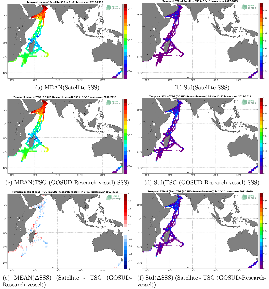
Figure 6: Temporal mean (left) and Std (right) of SSS from SMAP SSS L4 OI v1 - 7day (IPRC) (top), TSG (GOSUD-Research-vessel) (middle), and of \Delta SSS (Satellite - TSG (GOSUD-Research-vessel)). Only match-up pairs are used to generate these maps.
