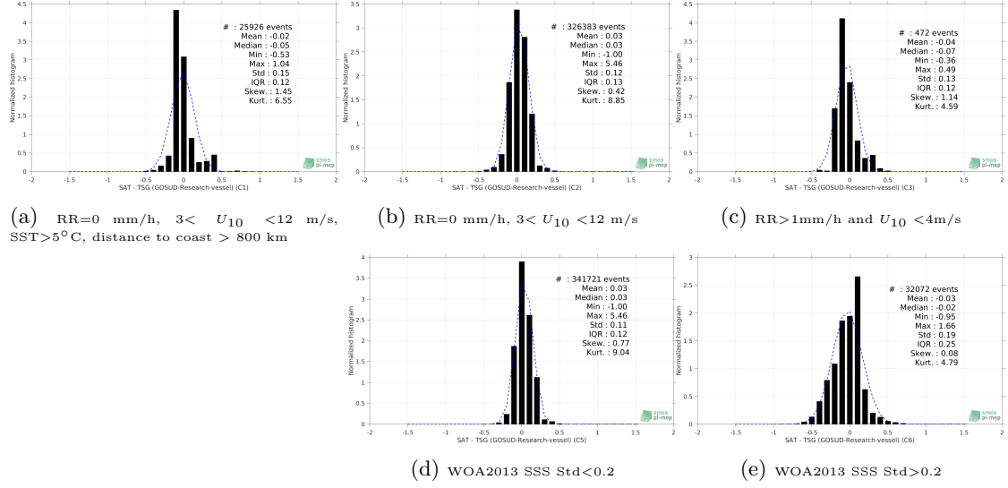
Figure 13: Normalized histogram of \Delta SSS (SMAP SSS L4 OI v1 - 7day (IPRC) - TSG (GOSUD-Research-vessel)) for 5 different subdatasets corresponding to: RR=0 mm/h, 3 < U_{10} < 12 m/s, SST>5°C, distance to coast > 800 km (a), RR=0 mm/h, 3 < U_{10} < 12 m/s (b), RR>1mm/h and U_{10} < 4 m/s (c), WOA2013 SSS Std<0.2 (d), WOA2013 SSS Std>0.2 (e).
