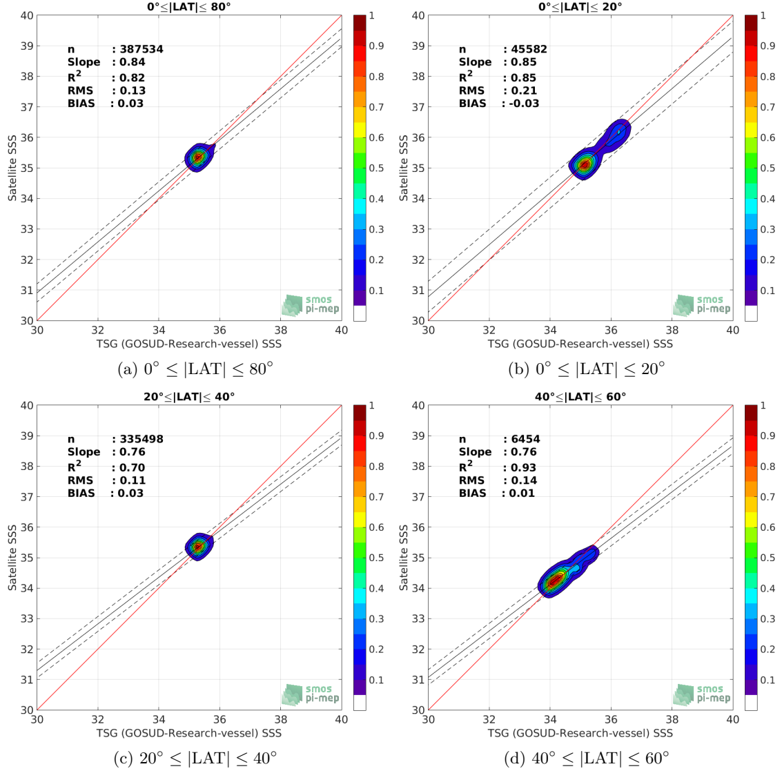
Figure 9: Contour maps of the concentration of SMAP SSS L4 OI v1 - 7day (IPRC) SSS (y-axis) versus TSG (GOSUD-Research-vessel) SSS (x-axis) at match-up pairs for different latitude bands. For each plot, the red line shows x=y . The black thin and dashed lines indicate a linear fit through the data cloud and the \pm 95\% confidence levels, respectively. The number match-up pairs n , the slope and R^2 coefficient of the linear fit, the root mean square (RMS) and the mean bias between satellite and in situ data are indicated for each latitude band in each plots.
