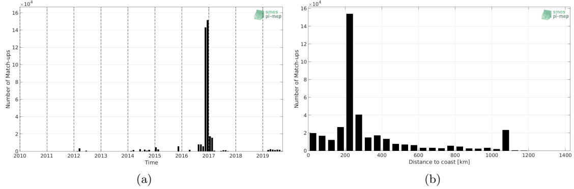
Figure 1: Number of match-ups between TSG (GOSUD-Research-vessel) and SMAP SSS L4 OI v1 - 7day (IPRC) SSS as a function of time (a) and as function of the distance to coast (b) over the Indian Ocean Pi-MEP region and for the full satellite product period.
