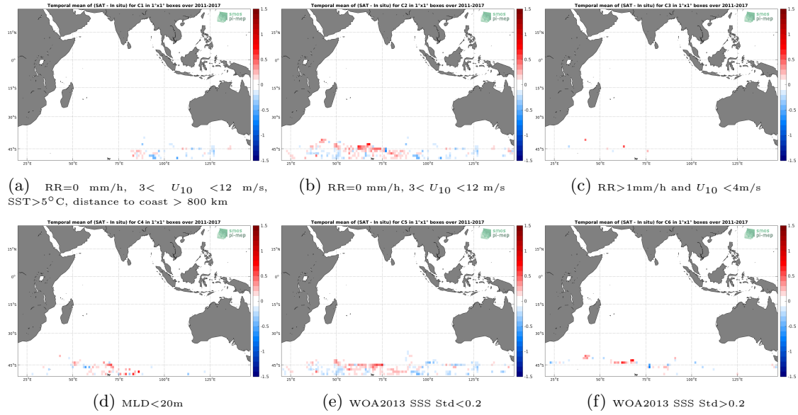
Figure 12: Temporal mean gridded over spatial boxes of size 1^{\circ} \times 1^{\circ} of \Delta\text{SSS} (SMAP SSS L4 OI v1 - 7 Days (IPRC) - Marine mammals) for 6 different subdatasets corresponding to: \text{RR}=0 mm/h, 3 < U_{10} < 12 m/s, \text{SST} > 5^{\circ}\text{C} , distance to coast > 800 km (a), \text{RR}=0 mm/h, 3 < U_{10} < 12 m/s (b), \text{RR} > 1\text{mm/h} and U_{10} < 4\text{m/s} (c), \text{MLD} < 20\text{m} (d), \text{WOA2013 SSS Std} < 0.2 (e), \text{WOA2013 SSS Std} > 0.2 (f).
