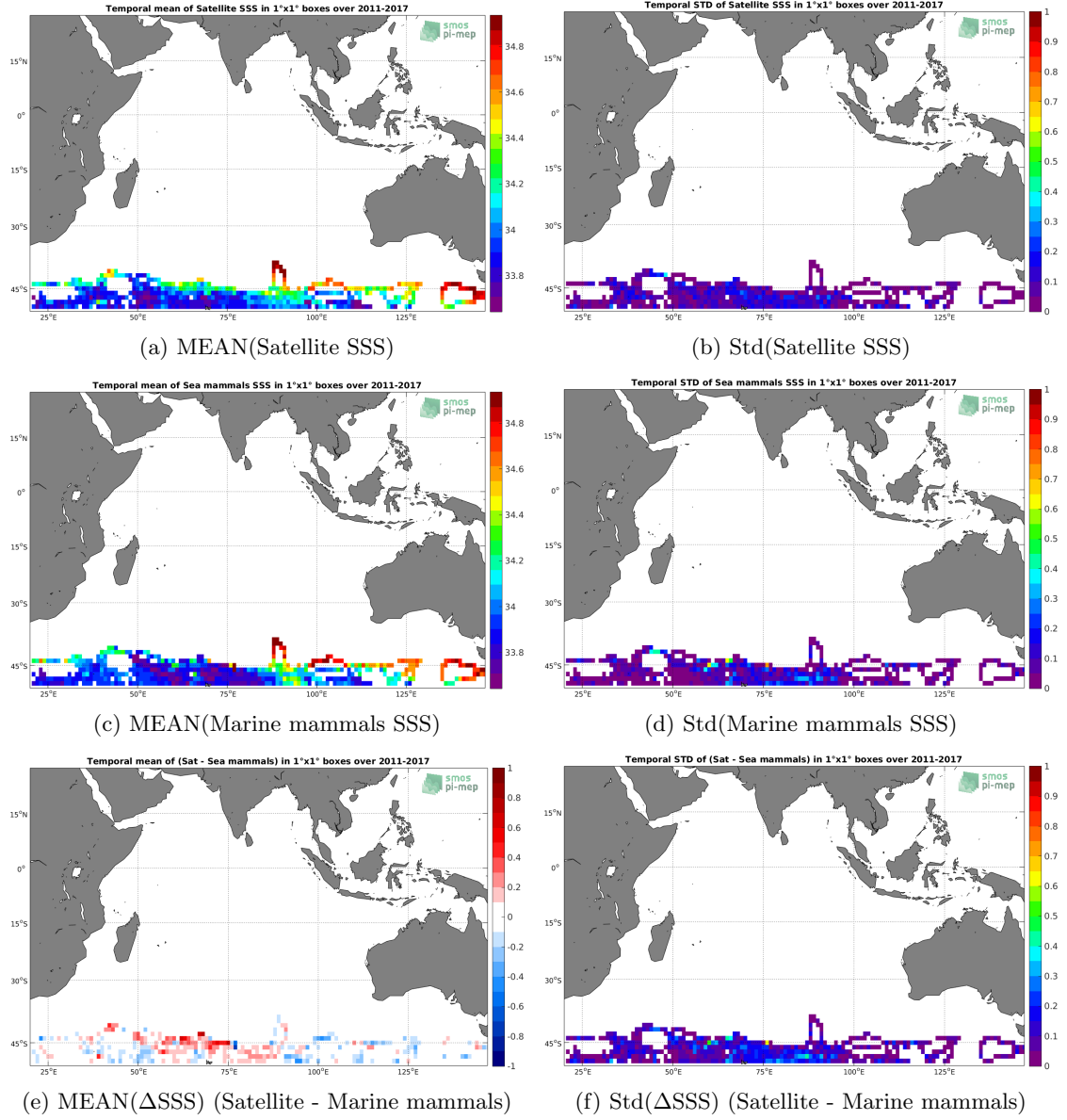
Figure 6: Temporal mean (left) and Std (right) of SSS from SMAP SSS L4 OI v1 - 7 Days (IPRC) (top), Marine mammals (middle), and of \Delta SSS (Satellite - Marine mammals). Only match-up pairs are used to generate these maps.
