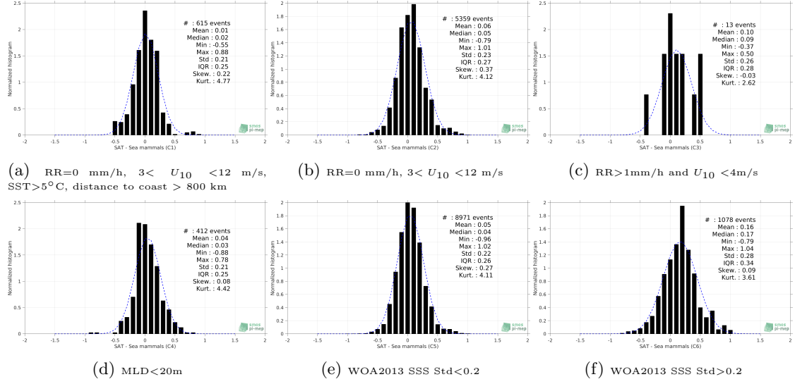
Figure 13: Normalized histogram of \Delta\text{SSS} (SMAP SSS L4 OI v1 - 7 Days (IPRC) - Marine mammals) for 6 different subdatasets corresponding to: RR=0 mm/h, 3 < U_{10} < 12 m/s, SST>5°C, distance to coast > 800 km (a), RR=0 mm/h, 3 < U_{10} < 12 m/s (b), RR>1mm/h and U_{10} < 4 m/s (c), MLD<20m (d), WOA2013 SSS Std<0.2 (e), WOA2013 SSS Std>0.2 (f).
