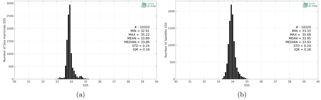
Figure 2: Histograms of SSS from Marine mammals (a) and SMAP SSS L4 OI v1 - 7 Days (IPRC) (b) considering all match-up pairs per bins of 0.1 over the Indian Ocean Pi-MEP region and for the full satellite product period.
