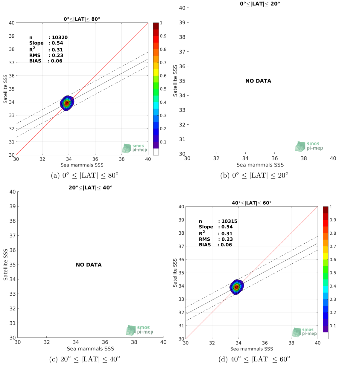
Figure 9: Contour maps of the concentration of SMAP SSS L4 OI v1 - 7day (IPRC) SSS (y-axis) versus Sea mammals SSS (x-axis) at match-up pairs for different latitude bands. For each plot, the red line shows x=y . The black thin and dashed lines indicate a linear fit through the data cloud and the \pm 95\% confidence levels, respectively. The number match-up pairs n , the slope and R^2 coefficient of the linear fit, the root mean square (RMS) and the mean bias between satellite and in situ data are indicated for each latitude band in each plots.
