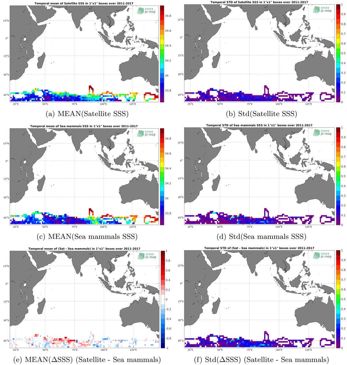
Figure 6: Temporal mean (left) and Std (right) of SSS from SMAP SSS L4 OI v1 - 7day (IPRC) (top), Sea mammals (middle), and of \Delta SSS (Satellite - Sea mammals). Only match-up pairs are used to generate these maps.
