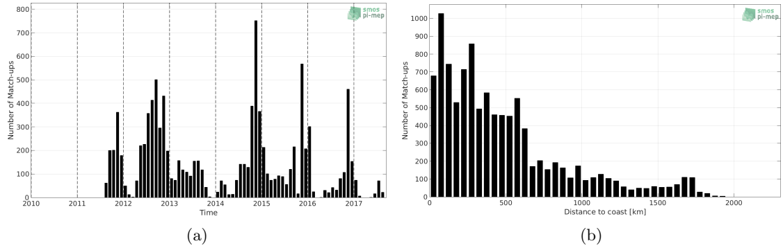
Figure 1: Number of match-ups between Sea mammals and SMAP SSS L4 OI v1 - 7day (IPRC) SSS as a function of time (a) and as function of the distance to coast (b) over the Indian Ocean Pi-MEP region and for the full satellite product period.
