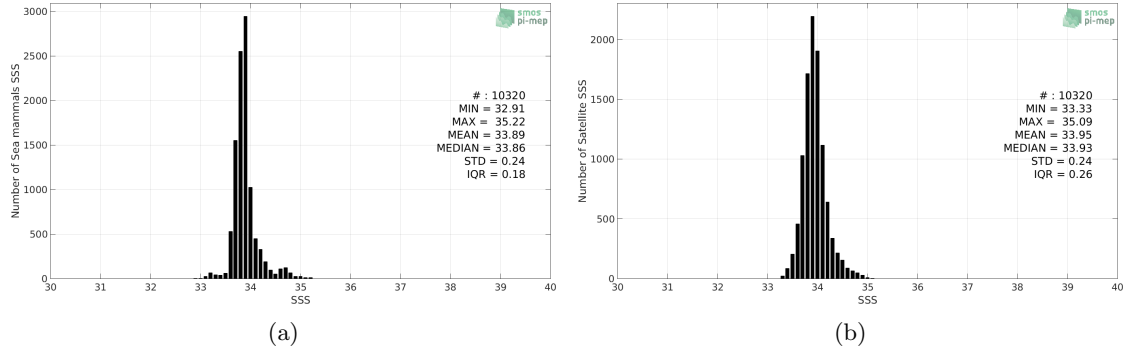
Figure 2: Histograms of SSS from Sea mammals (a) and SMAP SSS L4 OI v1 - 7day (IPRC) (b) considering all match-up pairs per bins of 0.1 over the Indian Ocean Pi-MEP region and for the full satellite product period.
