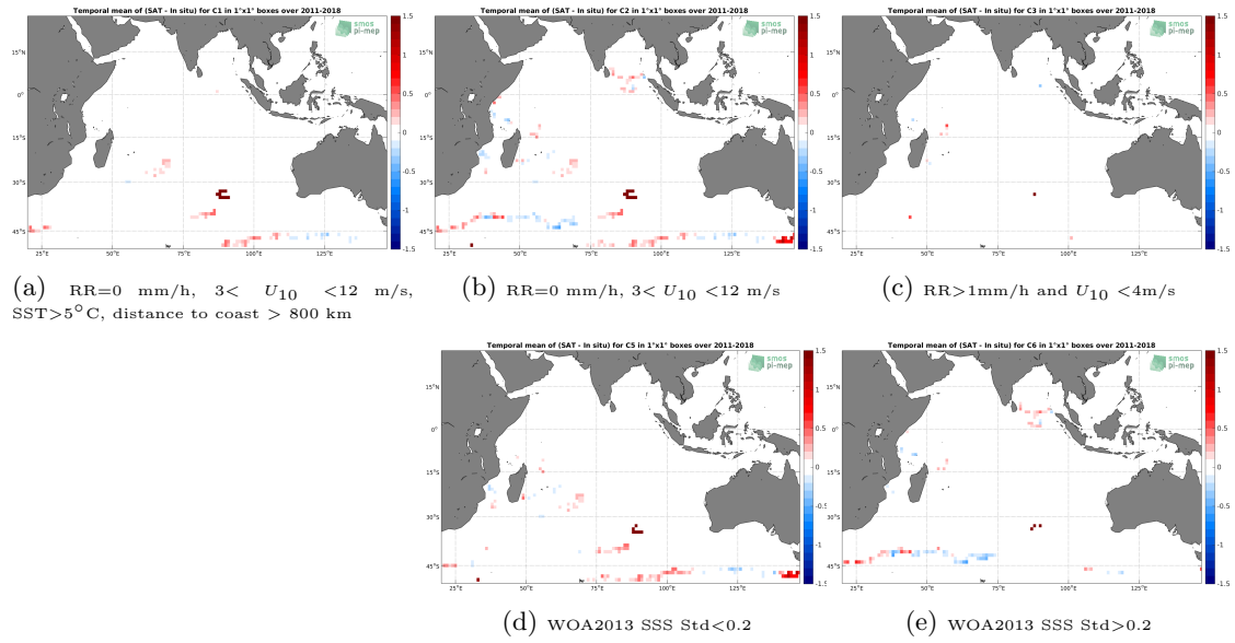
Figure 11: Temporal mean gridded over spatial boxes of size 1^\circ \times 1^\circ of \Delta SSS (SMAP SSS L4 OI v1 - 7 Days (IPRC) - Surface drifters) for 5 different subdatasets corresponding to: RR=0 mm/h, 3 < U_{10} < 12 m/s, SST > 5^\circ\text{C} , distance to coast > 800 km (a), RR=0 mm/h, 3 < U_{10} < 12 m/s (b), RR > 1\text{mm/h} and U_{10} < 4\text{m/s} (c), WOA2013 SSS Std < 0.2 (d), WOA2013 SSS Std > 0.2 (e).
