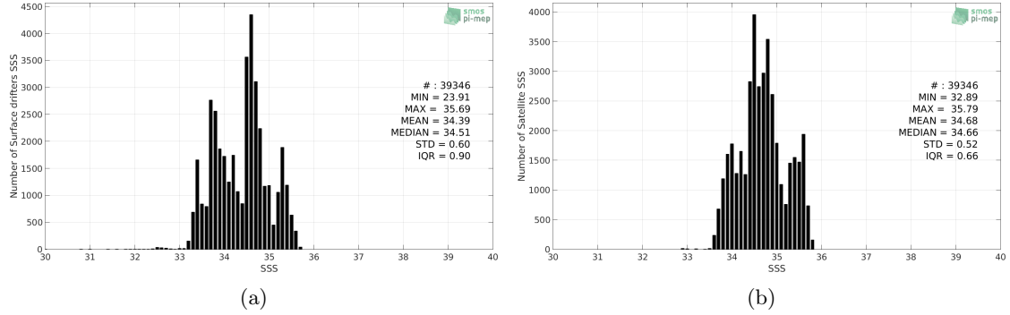
Figure 2: Histograms of SSS from Surface drifters (a) and SMAP SSS L4 OI v1 - 7 Days (IPRC) (b) considering all match-up pairs per bins of 0.1 over the Indian Ocean Pi-MEP region and for the full satellite product period.
