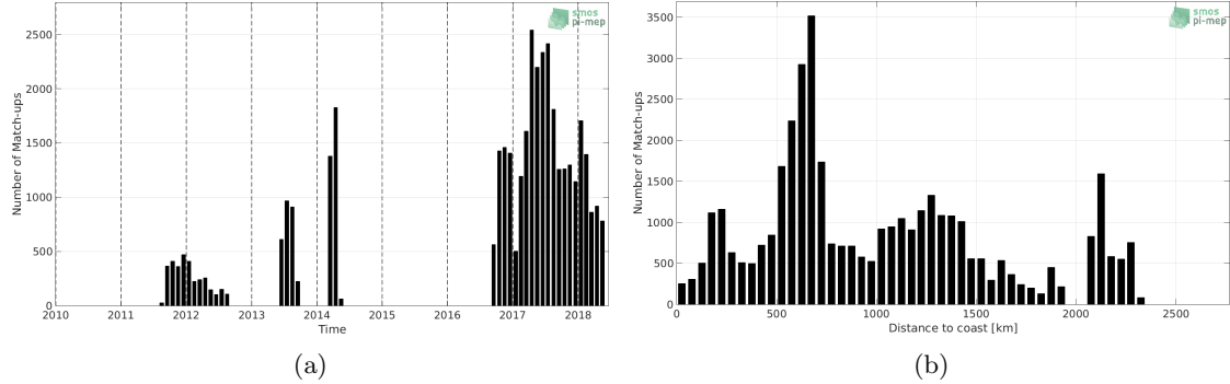
Figure 1: Number of match-ups between Surface drifters and SMAP SSS L4 OI v1 - 7 Days (IPRC) SSS as a function of time (a) and as function of the distance to coast (b) over the Indian Ocean Pi-MEP region and for the full satellite product period.
