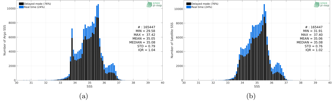
Figure 2: Histograms of SSS from Argo (a) and SMAP SSS L4 OI v1 - 7 Days (IPRC) (b) considering all match-up pairs per bins of 0.1 over the Indian Ocean Pi-MEP region and for the full satellite product period.
