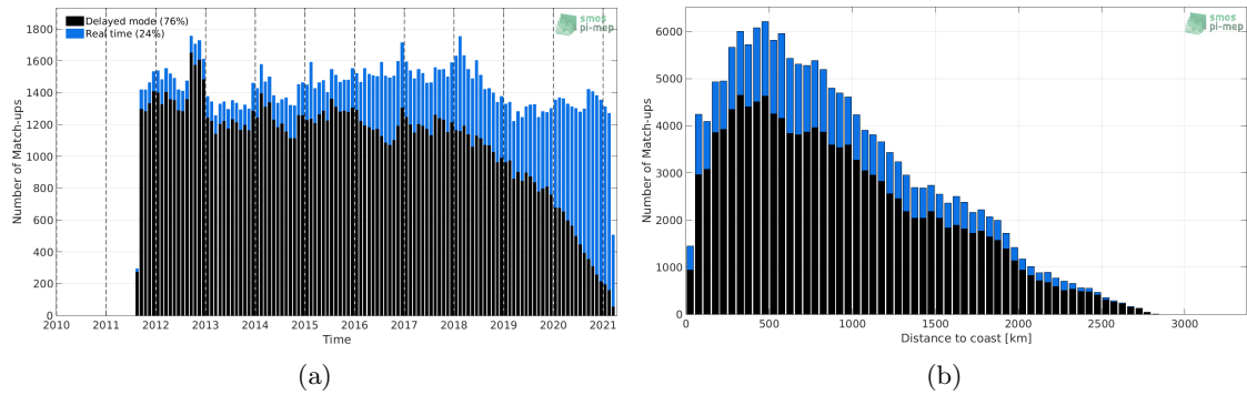
Figure 1: Number of match-ups between Argo and SMAP SSS L4 OI v1 - 7 Days (IPRC) SSS as a function of time (a) and as function of the distance to coast (b) over the Indian Ocean Pi-MEP region and for the full satellite product period.
