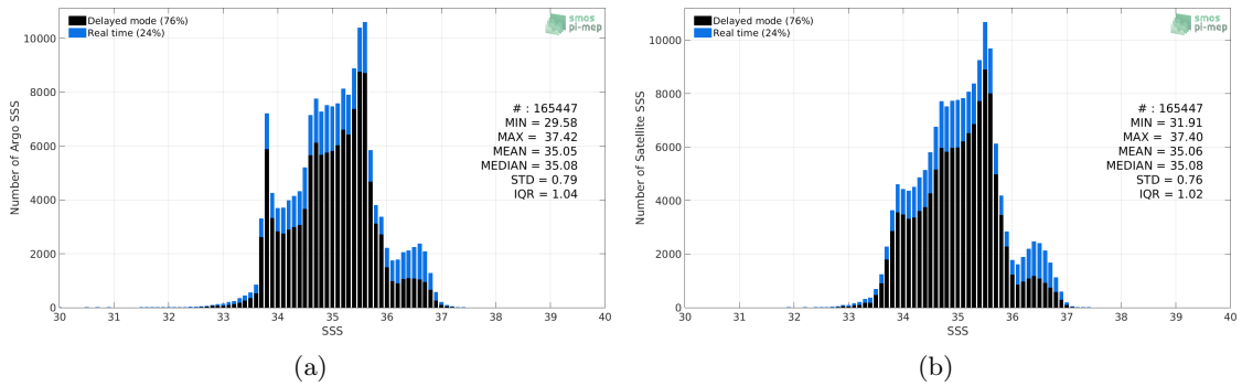
Figure 2: Histograms of SSS from Argo (a) and SMAP SSS L4 OI v1 - 7day (IPRC) (b) considering all match-up pairs per bins of 0.1 over the Indian Ocean Pi-MEP region and for the full satellite product period.
