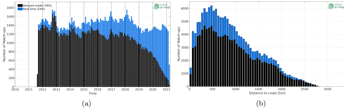
Figure 1: Number of match-ups between Argo and SMAP SSS L4 OI v1 - 7day (IPRC) SSS as a function of time (a) and as function of the distance to coast (b) over the Indian Ocean Pi-MEP region and for the full satellite product period.
