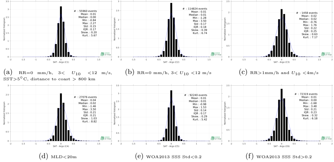
Figure 13: Normalized histogram of \Delta SSS (SMAP SSS L4 OI v1 - 7day (IPRC) - Argo) for 6 different subdatasets corresponding to: RR=0 mm/h, 3 < U_{10} < 12 m/s, SST>5°C, distance to coast > 800 km (a), RR=0 mm/h, 3 < U_{10} < 12 m/s (b), RR>1mm/h and U_{10} < 4 m/s (c), MLD<20m (d), WOA2013 SSS Std<0.2 (e), WOA2013 SSS Std>0.2 (f).
