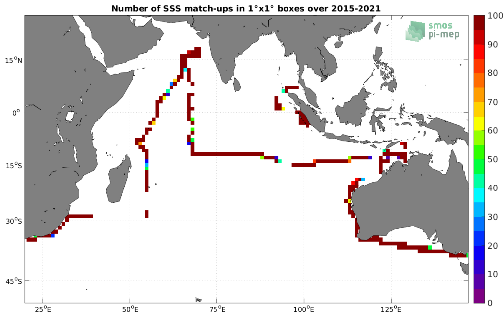
Figure 4: Number of SSS match-ups between TSG (SAMOS) SSS and the SMAP SSS L4 OI v1 - Monthly (IPRC) SSS product for the Indian Ocean Pi-MEP region over 1^\circ \times 1^\circ boxes and for the full satellite product period.
