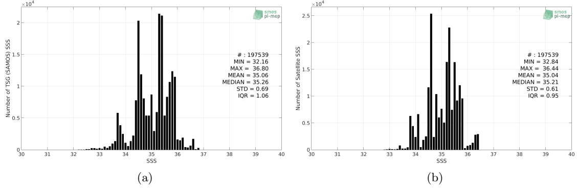
Figure 2: Histograms of SSS from TSG (SAMOS) (a) and SMAP SSS L4 OI v1 - Monthly (IPRC) (b) considering all match-up pairs per bins of 0.1 over the Indian Ocean Pi-MEP region and for the full satellite product period.
