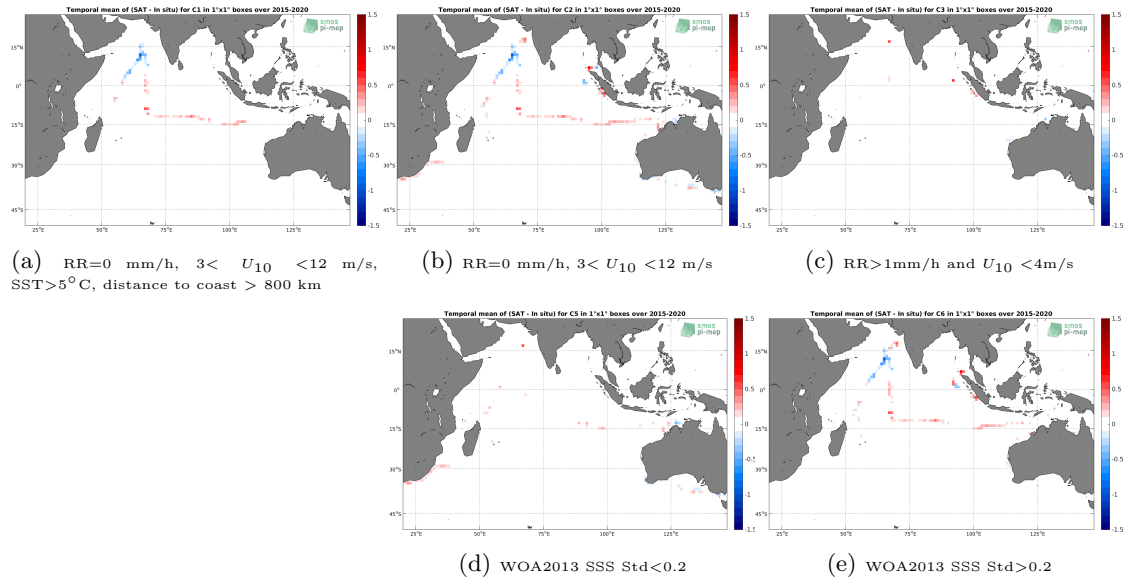
Figure 12: Temporal mean gridded over spatial boxes of size 1^\circ \times 1^\circ of \Delta SSS (SMAP SSS L4 OI v1 - Monthly (IPRC) - TSG (SAMOS)) for 5 different subdatasets corresponding to: RR=0 mm/h, 3 < U_{10} < 12 m/s, SST > 5^\circ C , distance to coast > 800 km (a), RR=0 mm/h, 3 < U_{10} < 12 m/s (b), RR > 1 mm/h and U_{10} < 4 m/s (c), WOA2013 SSS Std < 0.2 (d), WOA2013 SSS Std > 0.2 (e).
