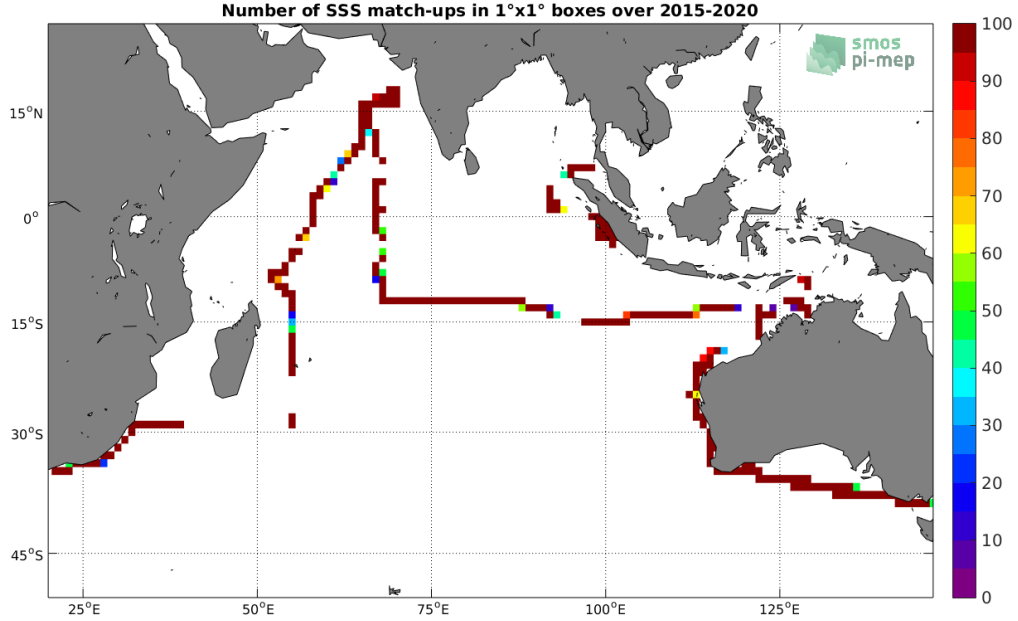
Figure 4: Number of SSS match-ups between TSG (SAMOS) SSS and the SMAP SSS L4 OI v1 - Monthly (IPRC) SSS product for the Indian Ocean Pi-MEP region over 1^\circ \times 1^\circ boxes and for the full satellite product period.
