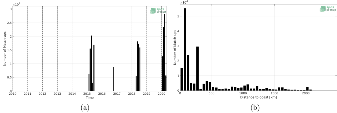
Figure 1: Number of match-ups between TSG (SAMOS) and SMAP SSS L4 OI v1 - Monthly (IPRC) SSS as a function of time (a) and as function of the distance to coast (b) over the Indian Ocean Pi-MEP region and for the full satellite product period.
