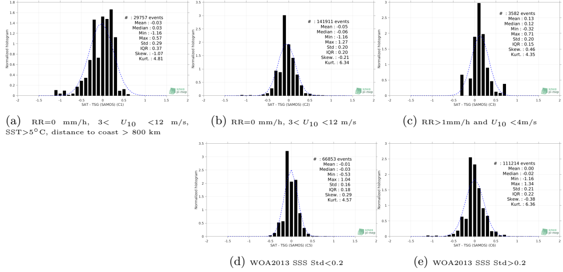
Figure 13: Normalized histogram of \Delta SSS (SMAP SSS L4 OI v1 - Monthly (IPRC) - TSG (SAMOS)) for 5 different subdatasets corresponding to: RR=0 mm/h, 3 < U_{10} < 12 m/s, SST>5°C, distance to coast > 800 km (a), RR=0 mm/h, 3 < U_{10} < 12 m/s (b), RR>1mm/h and U_{10} < 4 m/s (c), WOA2013 SSS Std<0.2 (d), WOA2013 SSS Std>0.2 (e).
