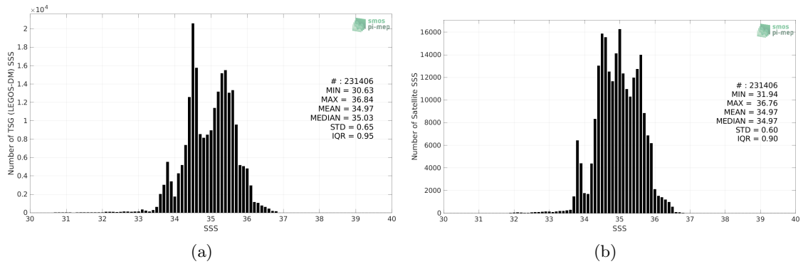
Figure 2: Histograms of SSS from TSG (LEGOS-DM) (a) and SMAP SSS L4 OI v1 - Monthly (IPRC) (b) considering all match-up pairs per bins of 0.1 over the Indian Ocean Pi-MEP region and for the full satellite product period.
