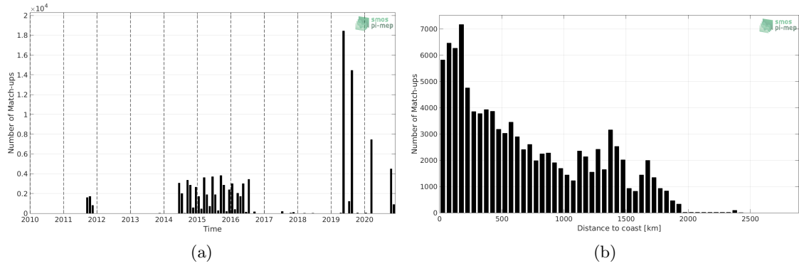
Figure 1: Number of match-ups between TSG (LEGOS-DM) and SMAP SSS L4 OI v1 - Monthly (IPRC) SSS as a function of time (a) and as function of the distance to coast (b) over the Indian Ocean Pi-MEP region and for the full satellite product period.
