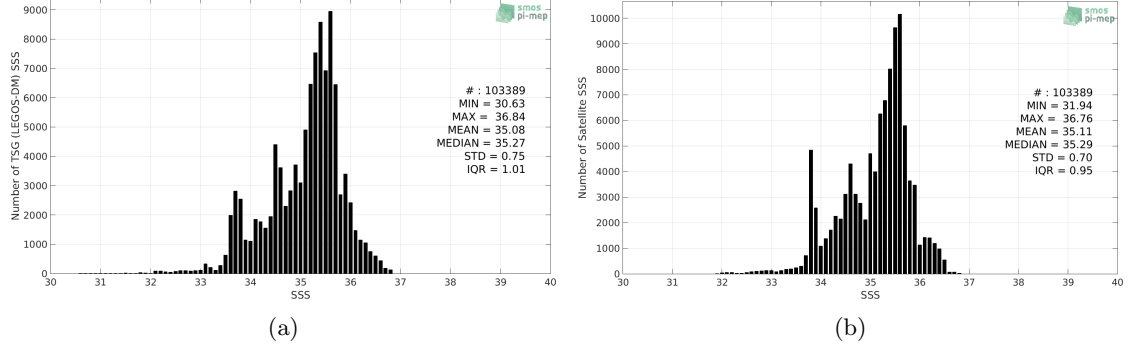
Figure 2: Histograms of SSS from TSG (LEGOS-DM) (a) and SMAP SSS L4 OI v1 - Monthly (IPRC) (b) considering all match-up pairs per bins of 0.1 over the Indian Ocean Pi-MEP region and for the full satellite product period.
