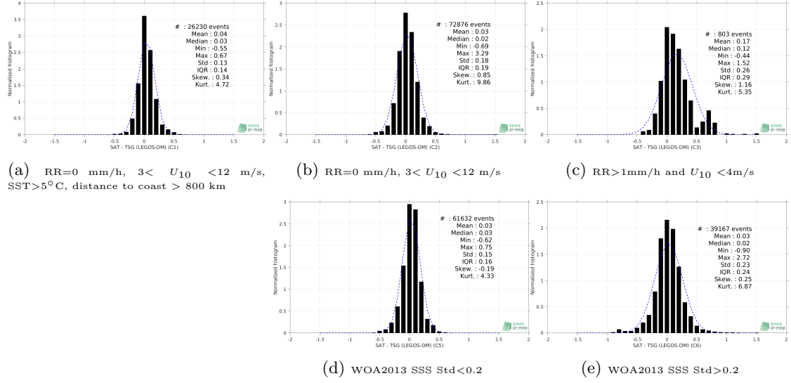
Figure 13: Normalized histogram of \Delta\text{SSS} (SMAP SSS L4 OI v1 - Monthly (IPRC) - TSG (LEGOS-DM)) for 5 different subdatasets corresponding to: RR=0 mm/h, 3 < U_{10} < 12 m/s, SST>5°C, distance to coast > 800 km (a), RR=0 mm/h, 3 < U_{10} < 12 m/s (b), RR>1mm/h and U_{10} < 4 m/s (c), WOA2013 SSS Std<0.2 (d), WOA2013 SSS Std>0.2 (e).
