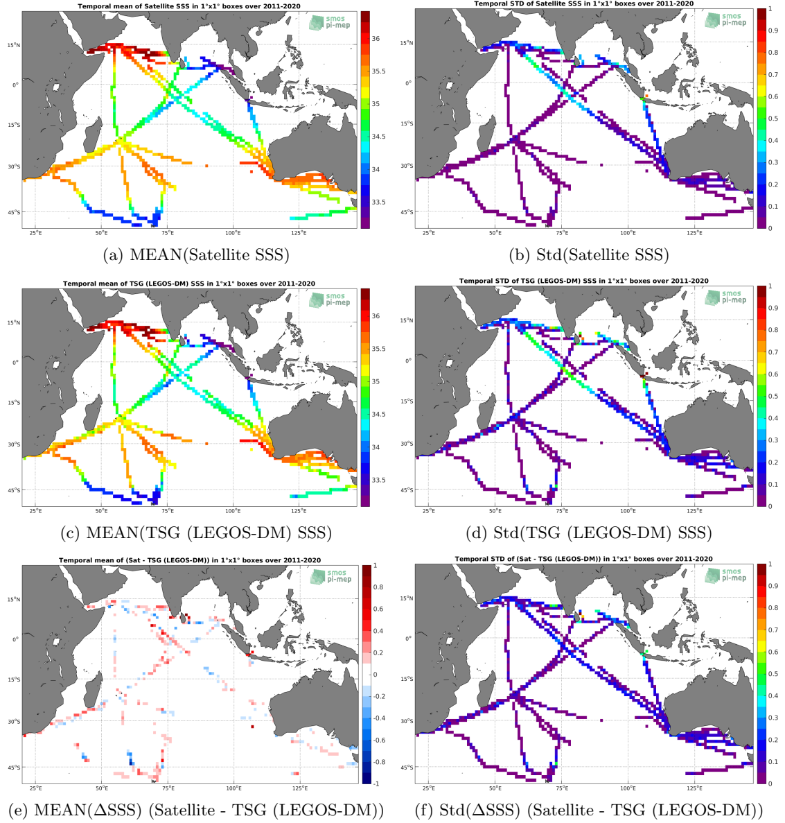
Figure 6: Temporal mean (left) and Std (right) of SSS from SMAP SSS L4 OI v1 - Monthly (IPRC) (top), TSG (LEGOS-DM) (middle), and of \Delta SSS (Satellite - TSG (LEGOS-DM)). Only match-up pairs are used to generate these maps.
